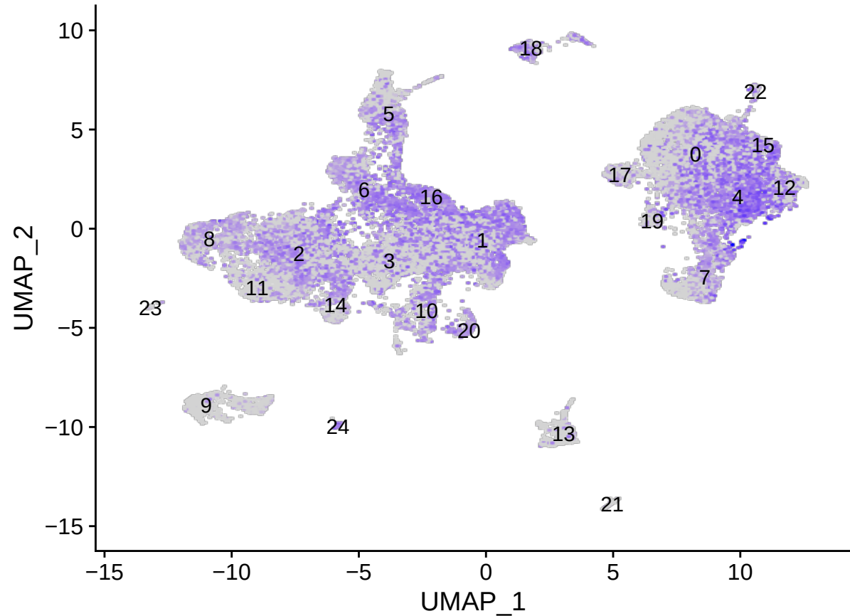
S100B
