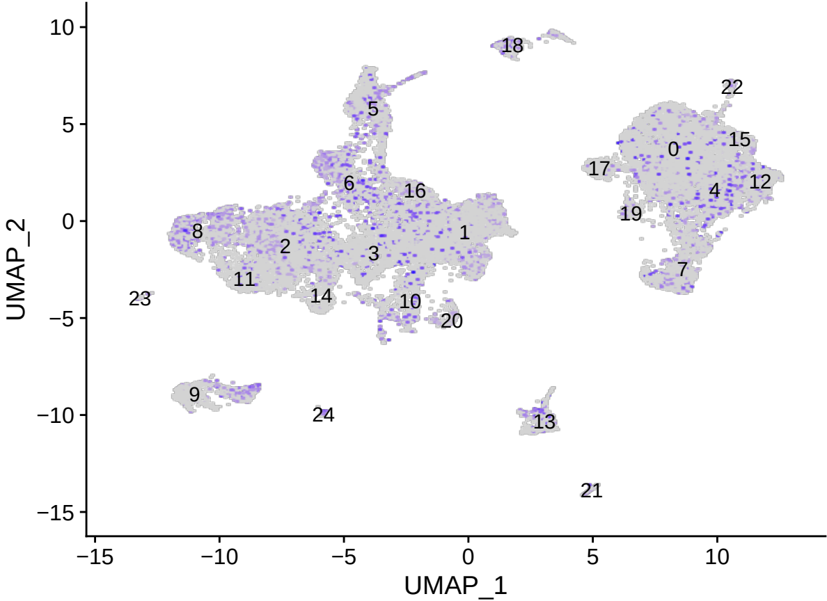
FTH1
