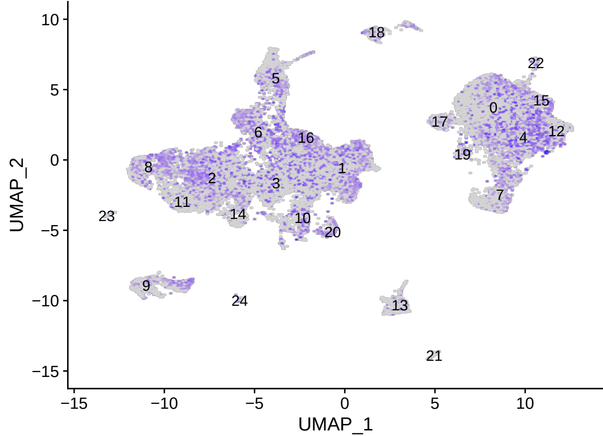
CD81
