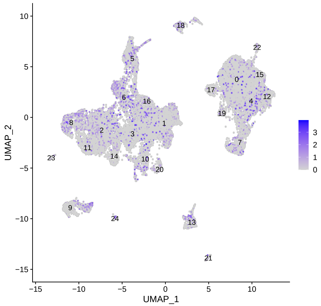
C1QB
