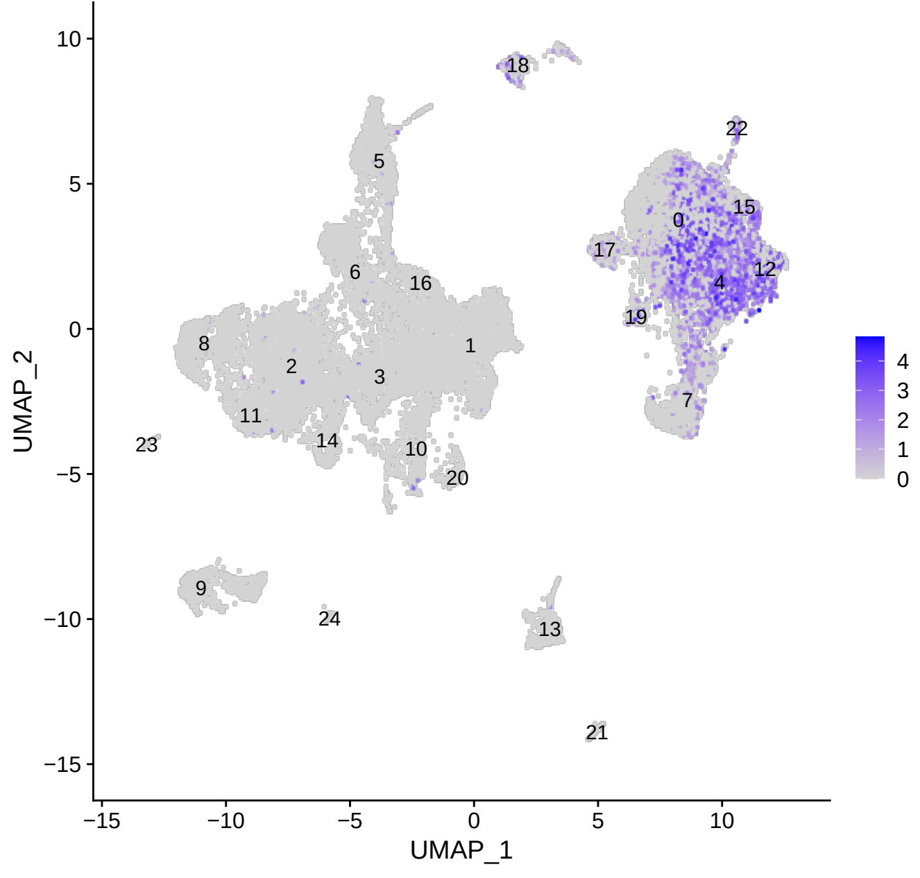
C1QC
