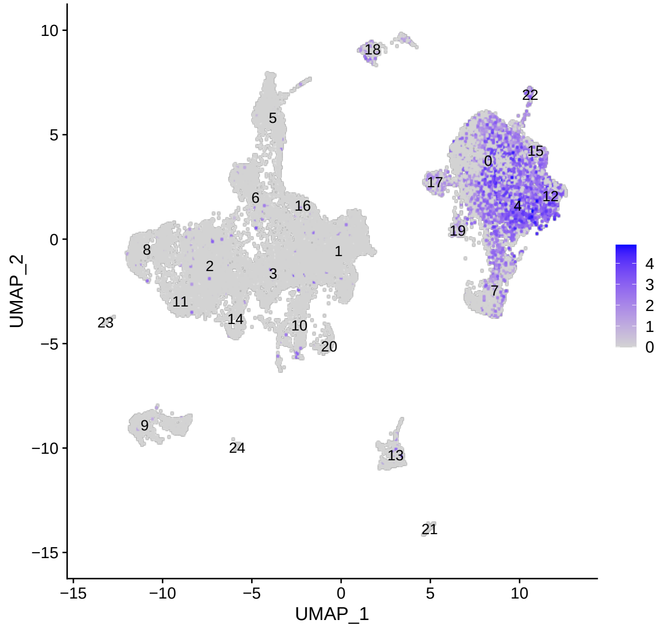
C1QC
