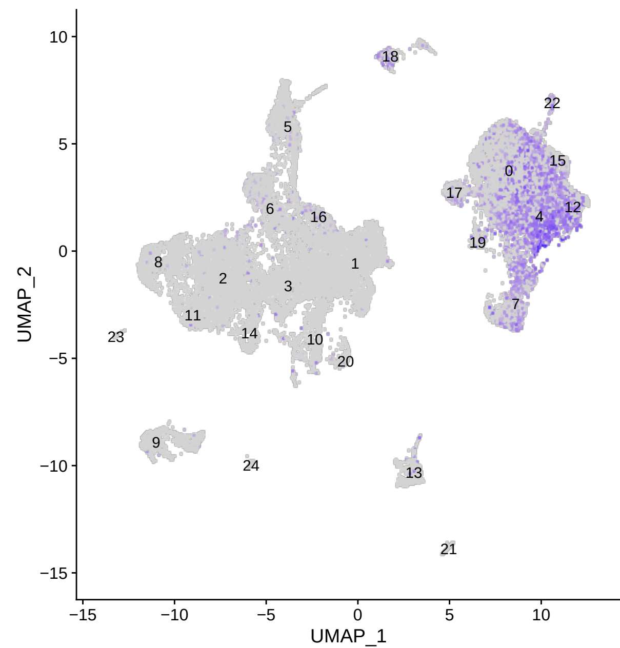
CD74
