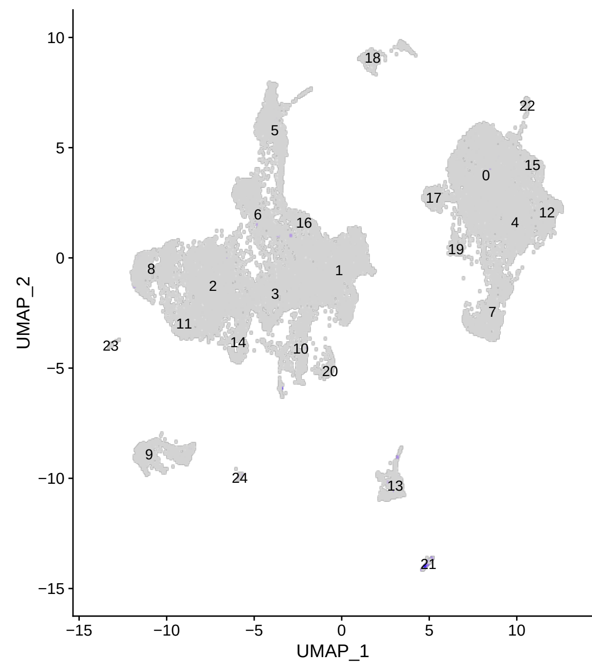
IGHM
