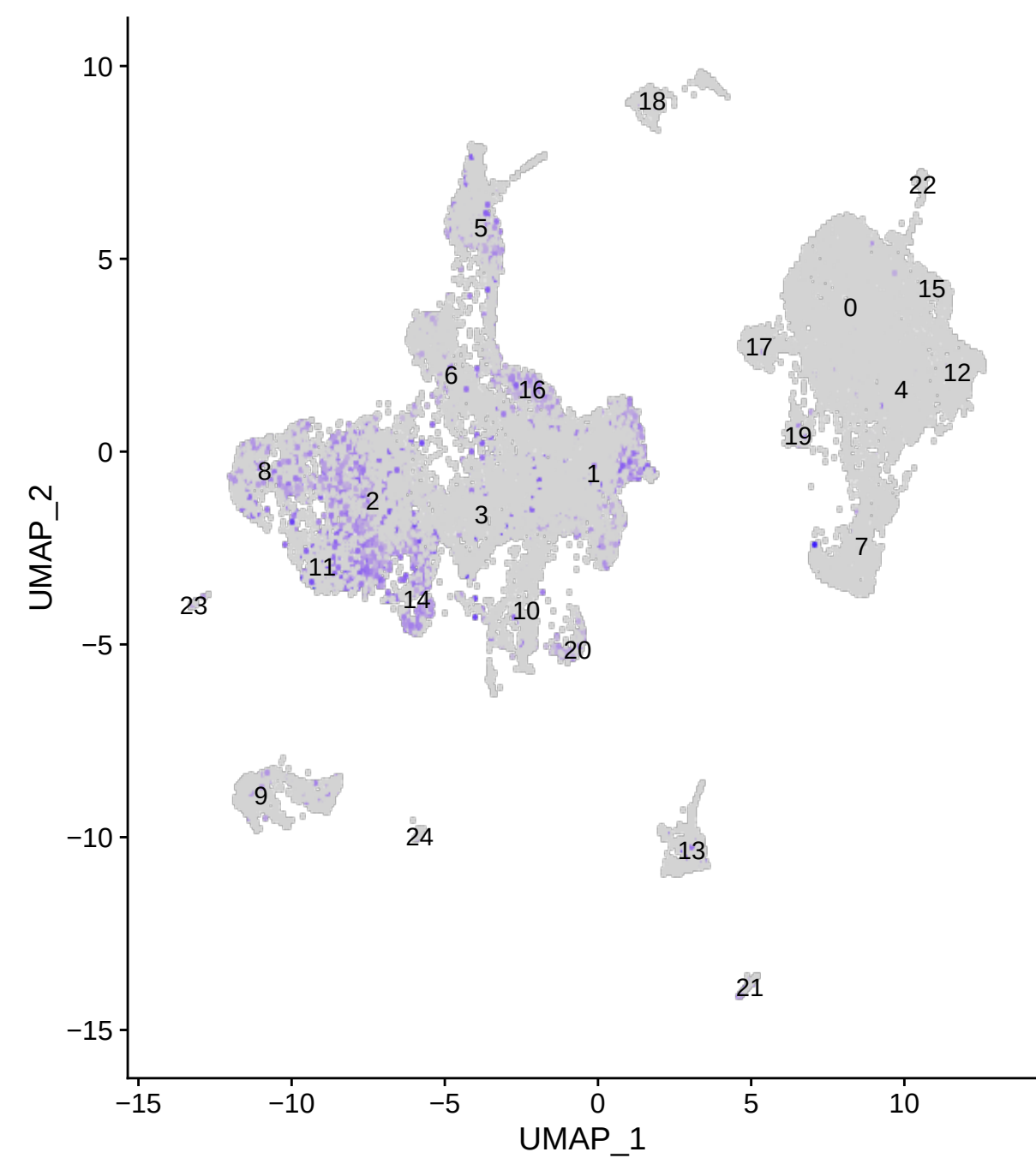
IGHM
