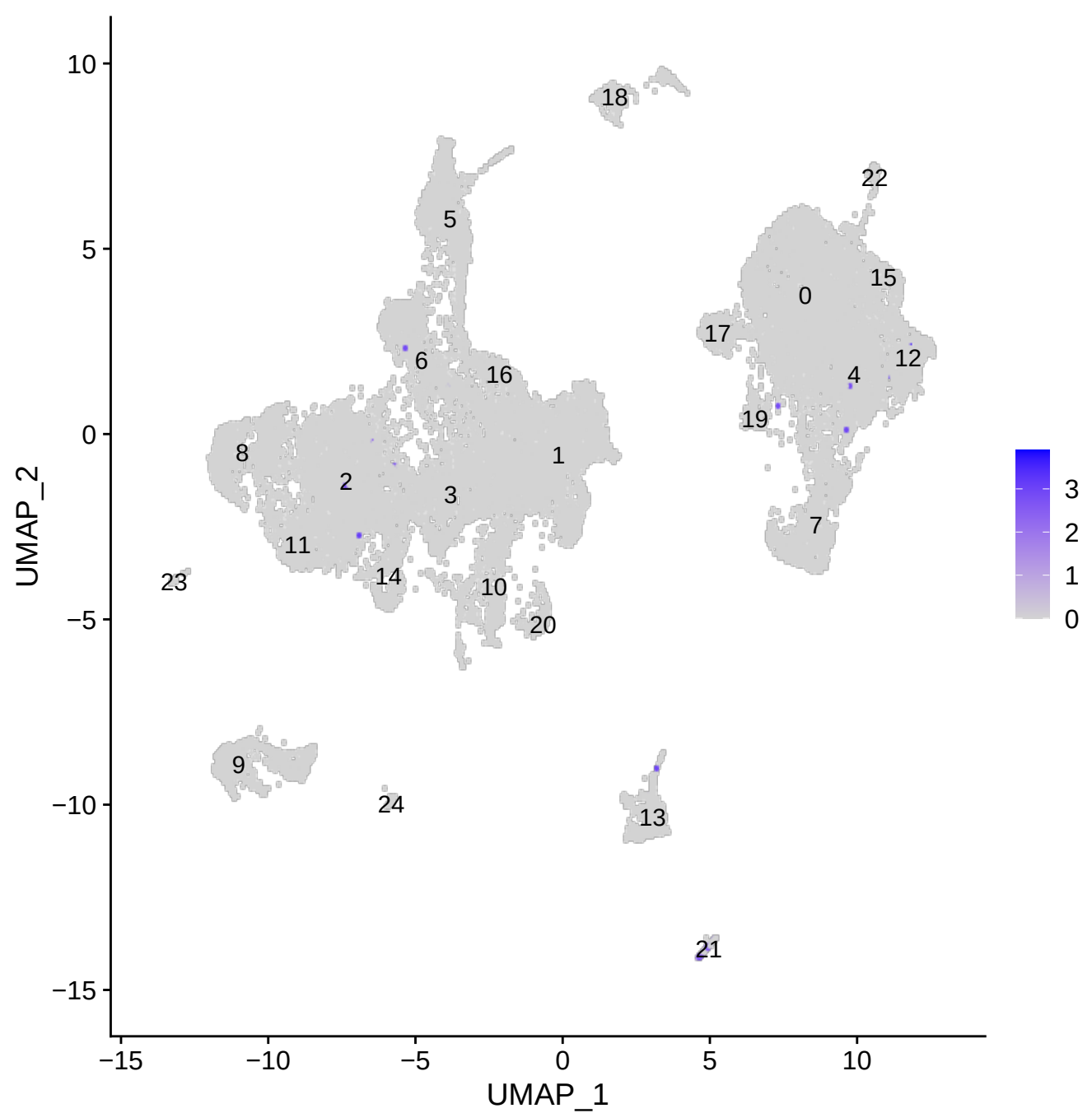
CD79A
