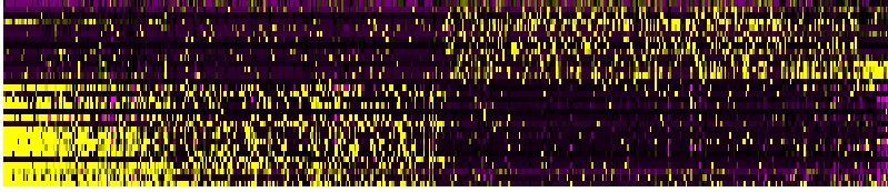
PC_19
