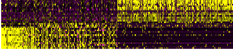
PC_18
