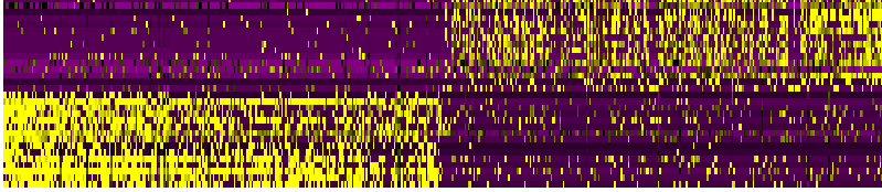
PC_16
