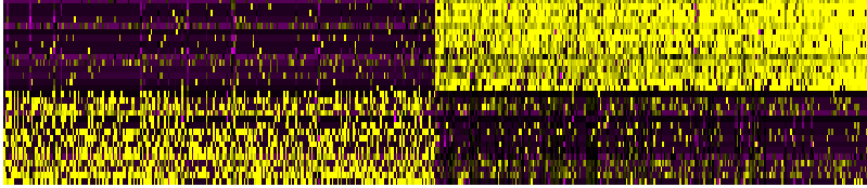
PC_10
