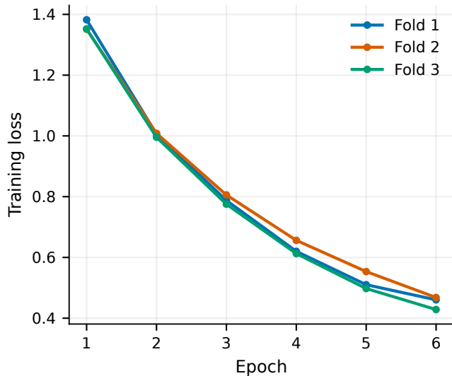
(a) Training
