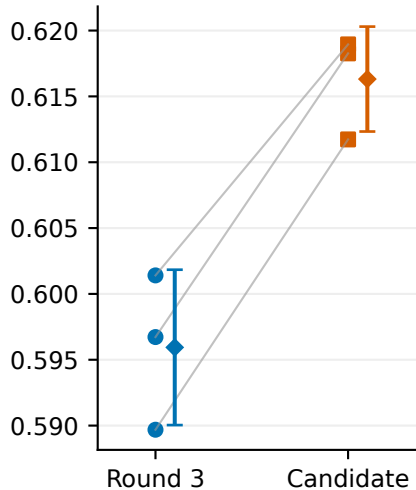
(a) Clean Macro-F1
