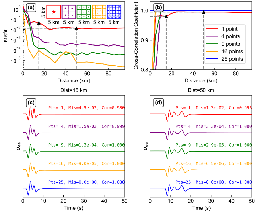
Figure 10. Discretization errors associated with subfault sampling. A 5 km \times 5 km subfault is represented either by a single point source or by 4, 9, 16, and 25 uniformly distributed points (schematic in panel a). All points share the same focal mechanism, (strike, dip, rake) = (0°, 90°, 0°). The subfault center lies at 10 km depth; the receiver is located northeast of the subfault center (azimuth 45°) at a depth of 1 km. Waveform differences are evaluated relative to the highest sampling (25 points) as epicentral distance increases. (a) Misfit versus epicentral distance. (b) Cross-correlation coefficient versus epicentral distance. (c) \sigma_{ee} stress component for different numbers of discretization points at an epicentral distance of 15 km. (d) \sigma_{ee} stress component for different numbers of discretization points at an epicentral distance of 50 km.
