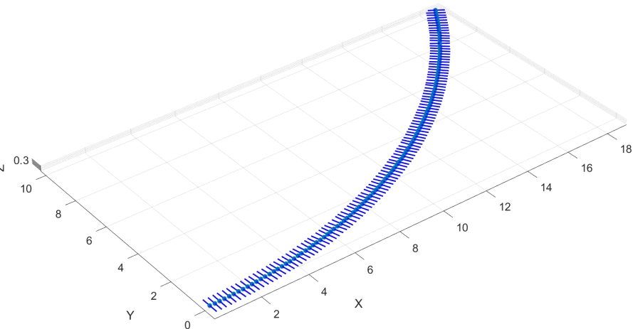
ASCM Results
