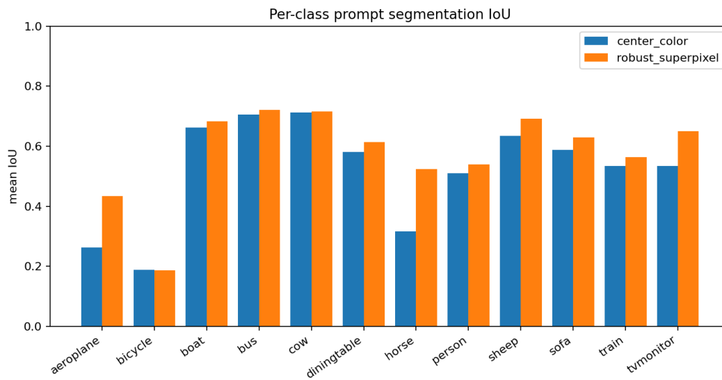
Figure 2: Per-class mean IoU. The strongest gains appear on horse, tvmmonitor, and aeroplane examples.
