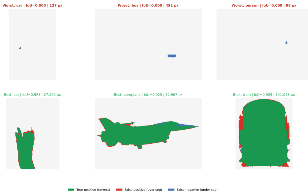
Figure 4: Error maps for three worst and three best Robust Superpixel predictions. Green = true positive, red = false positive, blue = false negative. Worst cases (top row) are dominated by thin structures and small targets; best cases (bottom row) are large, uniformly coloured objects.
