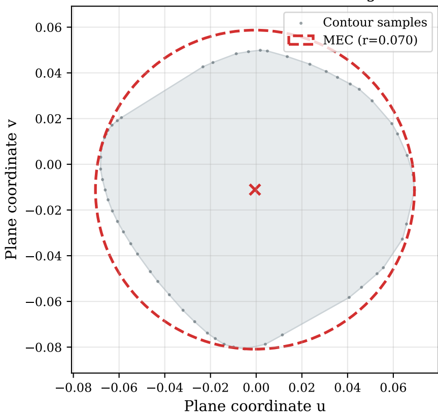
(c) Cross-section 5 with fitted covering circle
