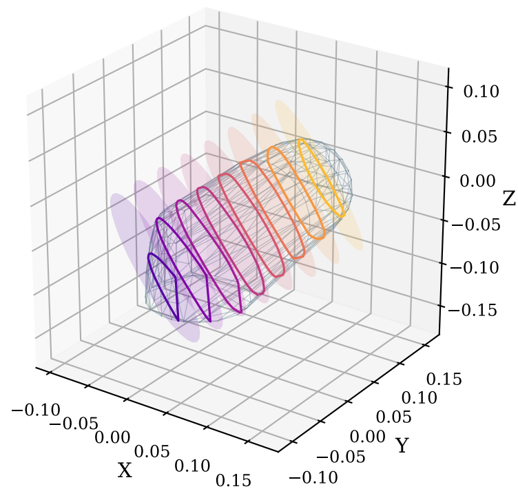
(b) Cross-section planes
