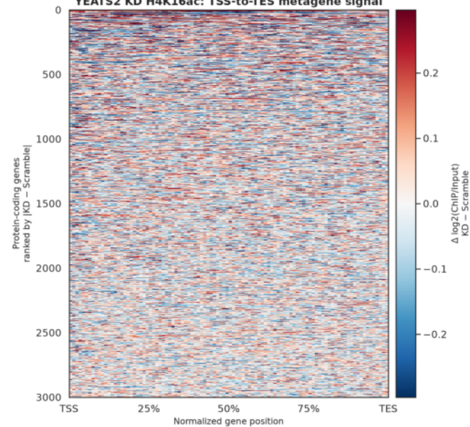
YEATS2 KD H4K16ac: TSS-to-TES metagene signal
