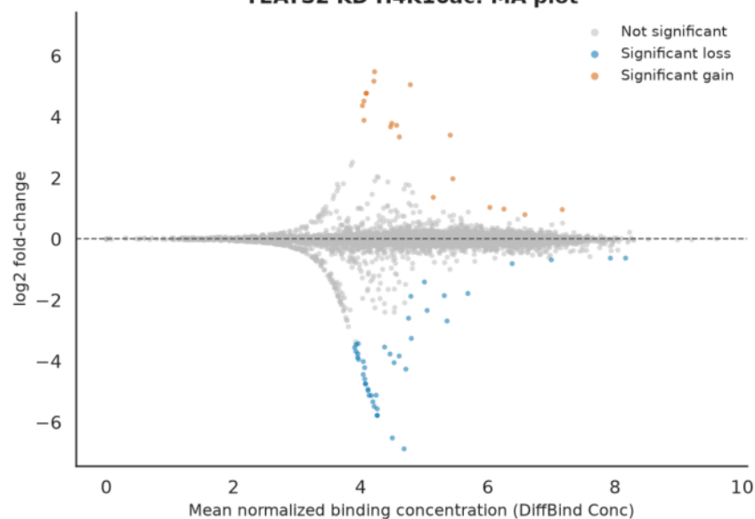
YEATS2 KD H4K16ac: MA plot
