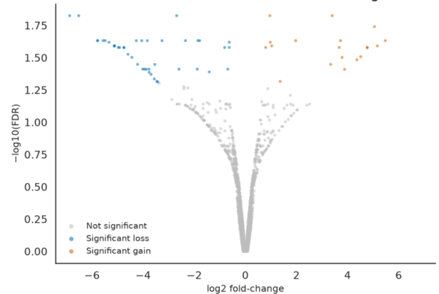
YEATS2 KD H4K16ac: differential binding
