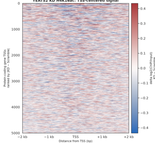
YEATS2 KD H4K16ac: TSS-centered signal
