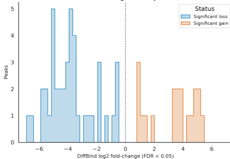
YEATS2 KD H4K16ac: significant peak effect sizes
