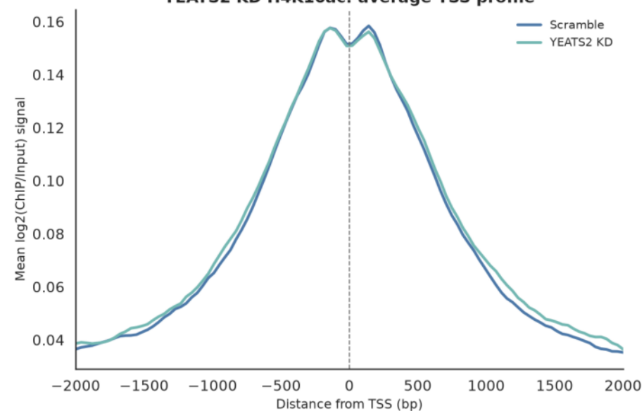
YEATS2 KD H4K16ac: average TSS profile
