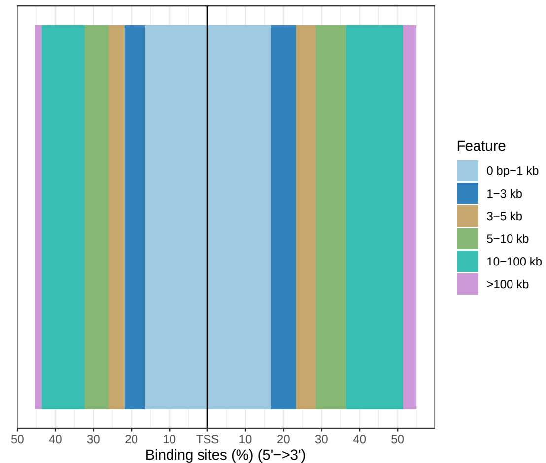
yeats2kd2
