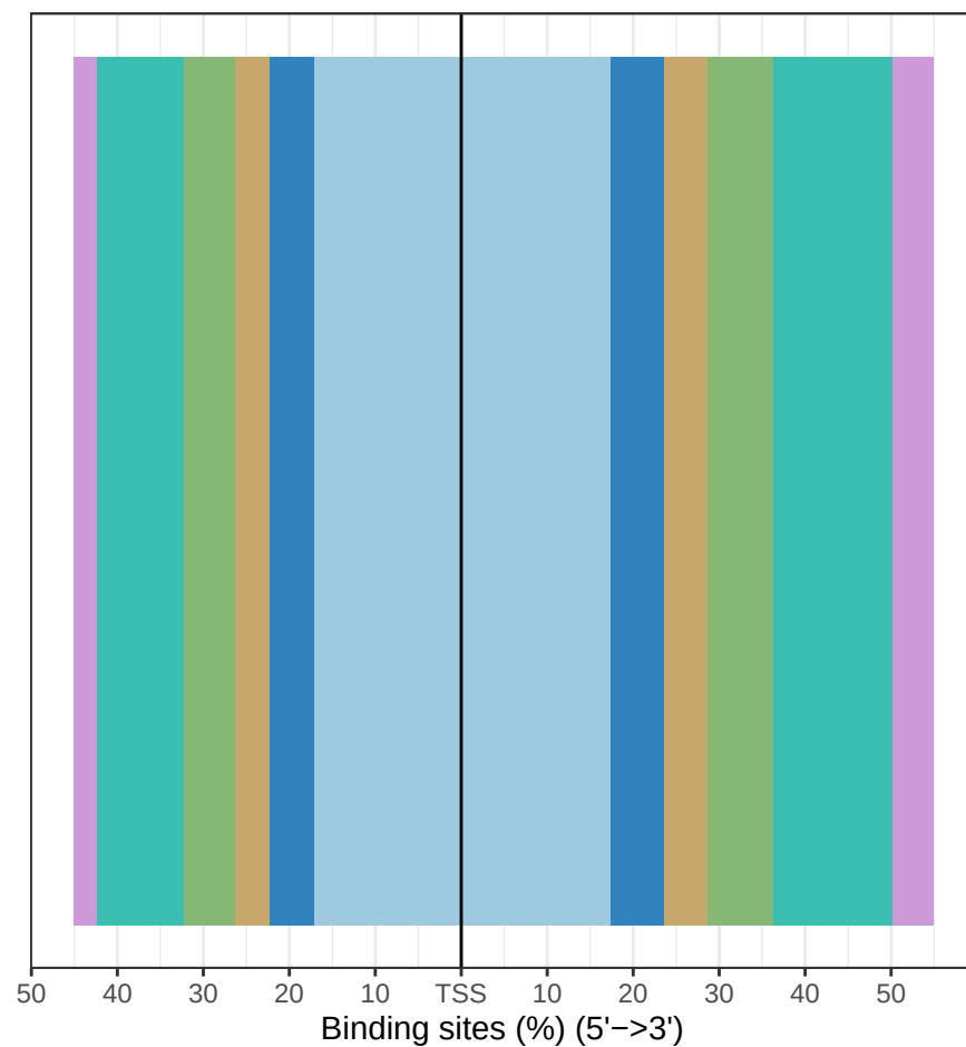
yeats2kd1
