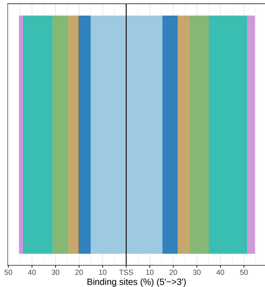
scramble1
