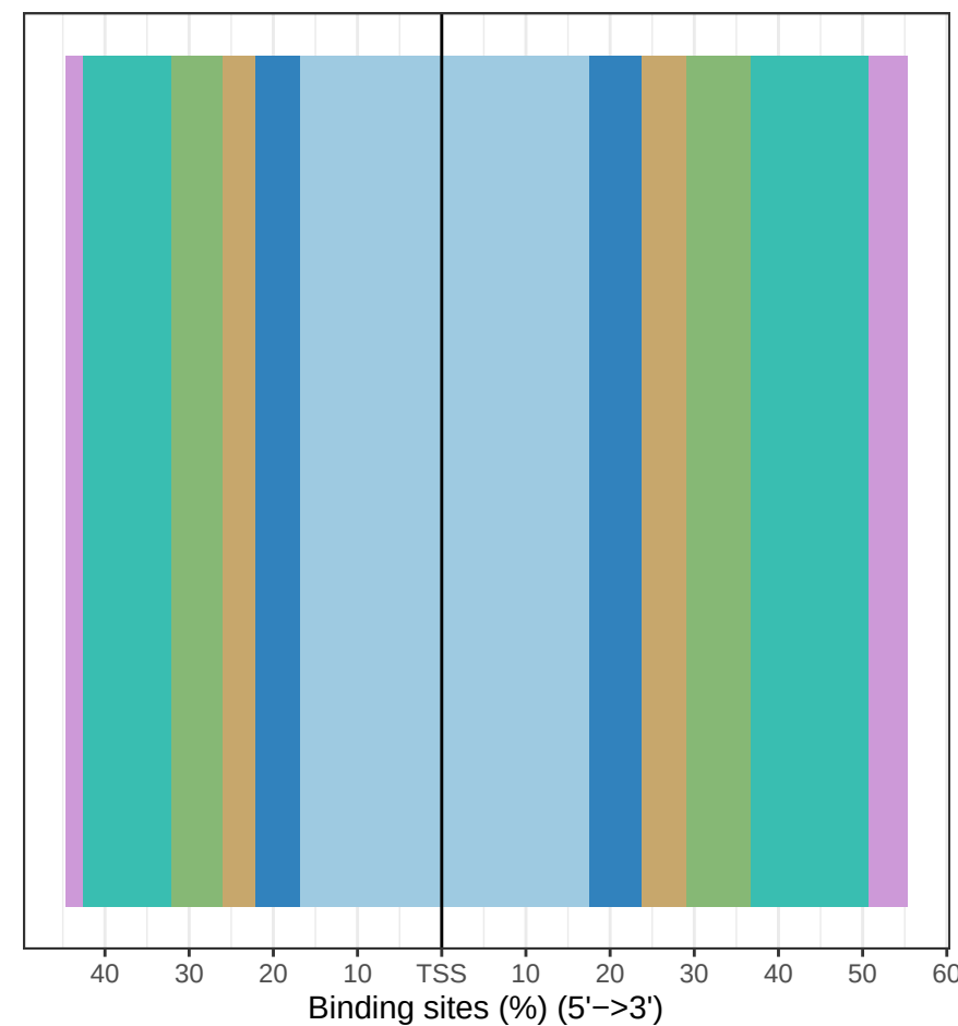
scramble2
