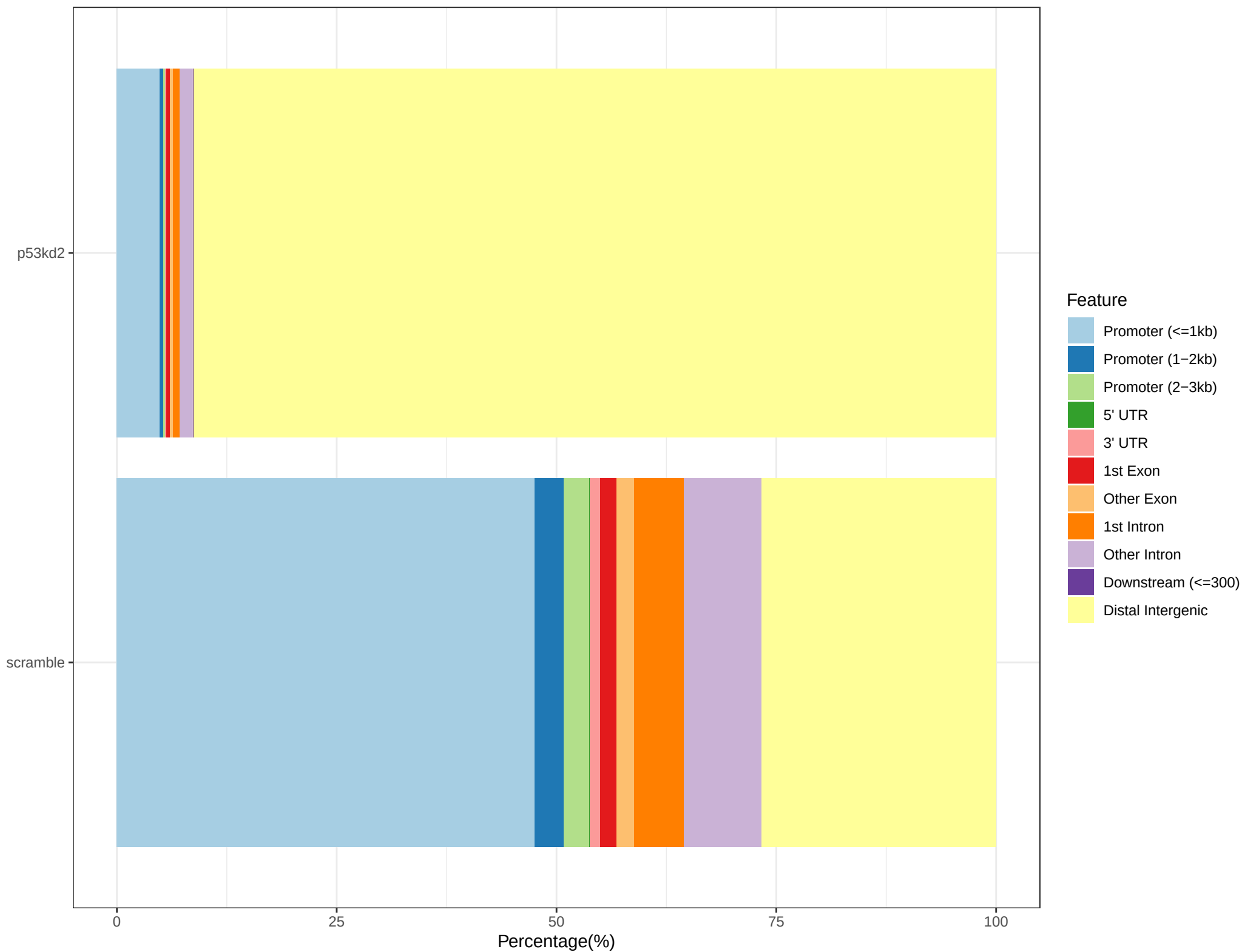
Feature Distribution
