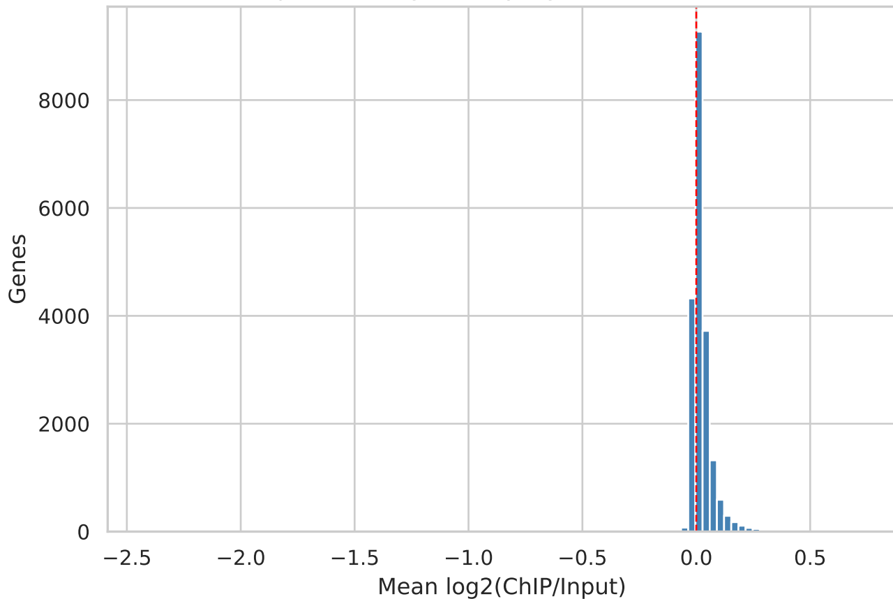
p53 0-hour genebody signal distribution
