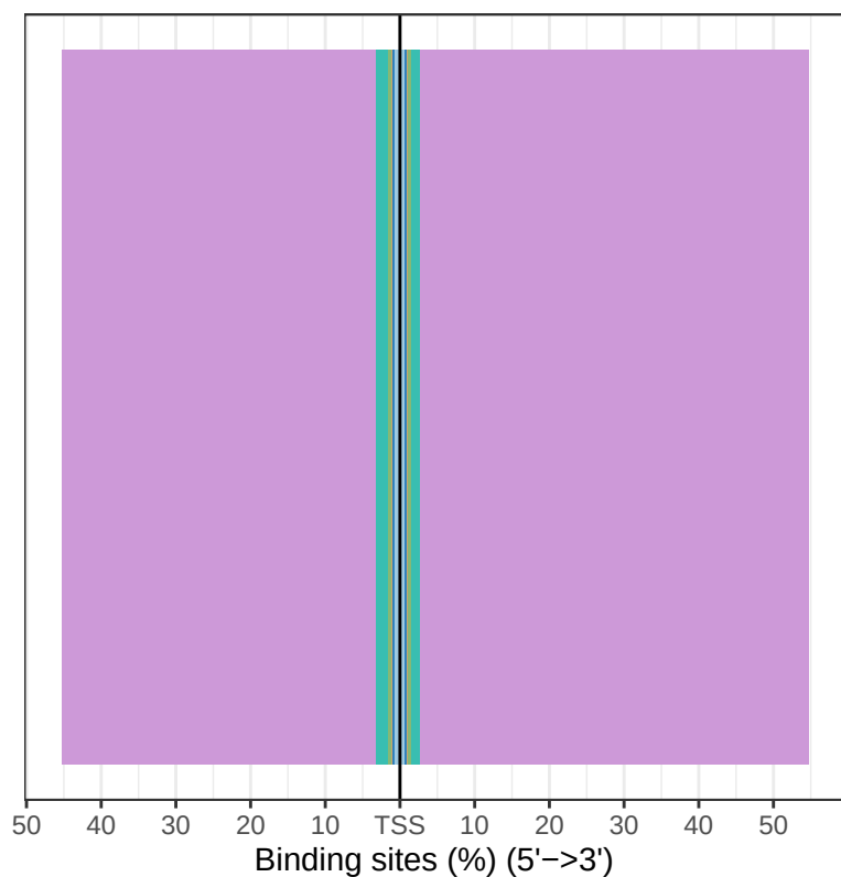
Scr_MOF_consensus
