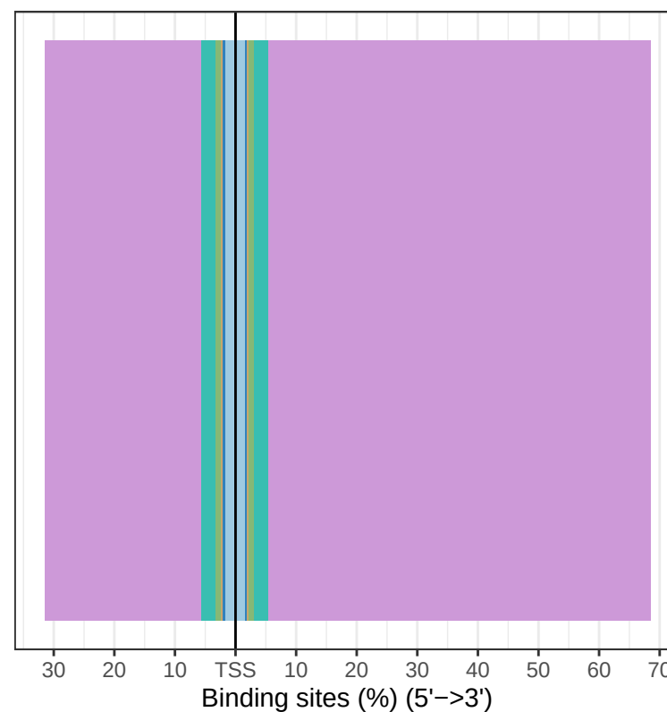
p53sh_MOF_consensus
