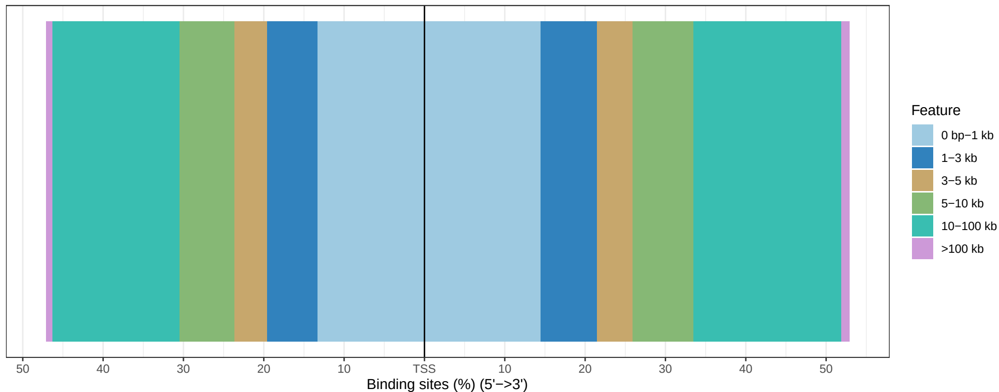
p53_0hr
