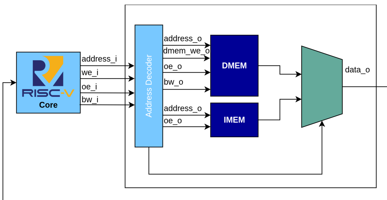
Figure 3. Address Decoder Block Diagram
