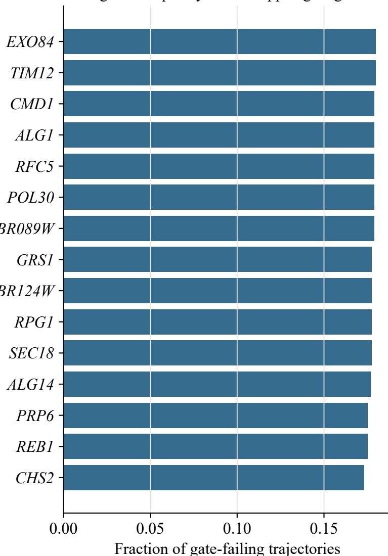
a Highest-frequency exact-mapped gate genes
