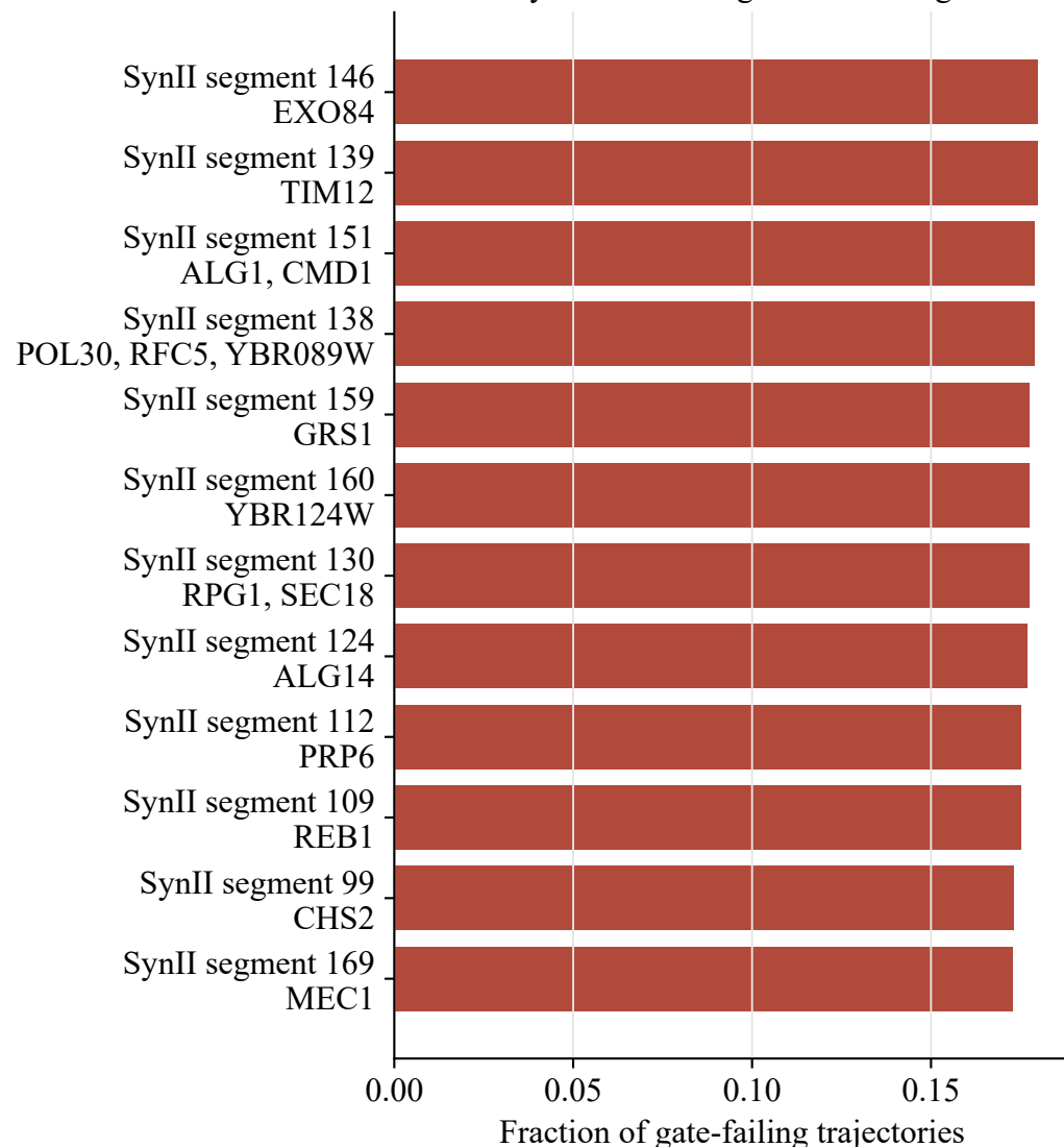
b Recurrently lost essential-gene-containing intervals
