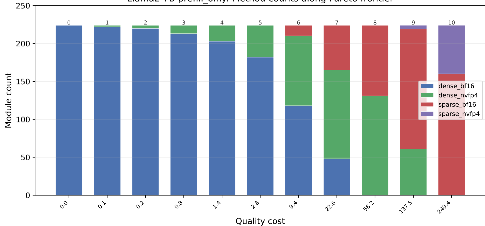
Llama2-7B prefill_only: Method counts along Pareto frontier
