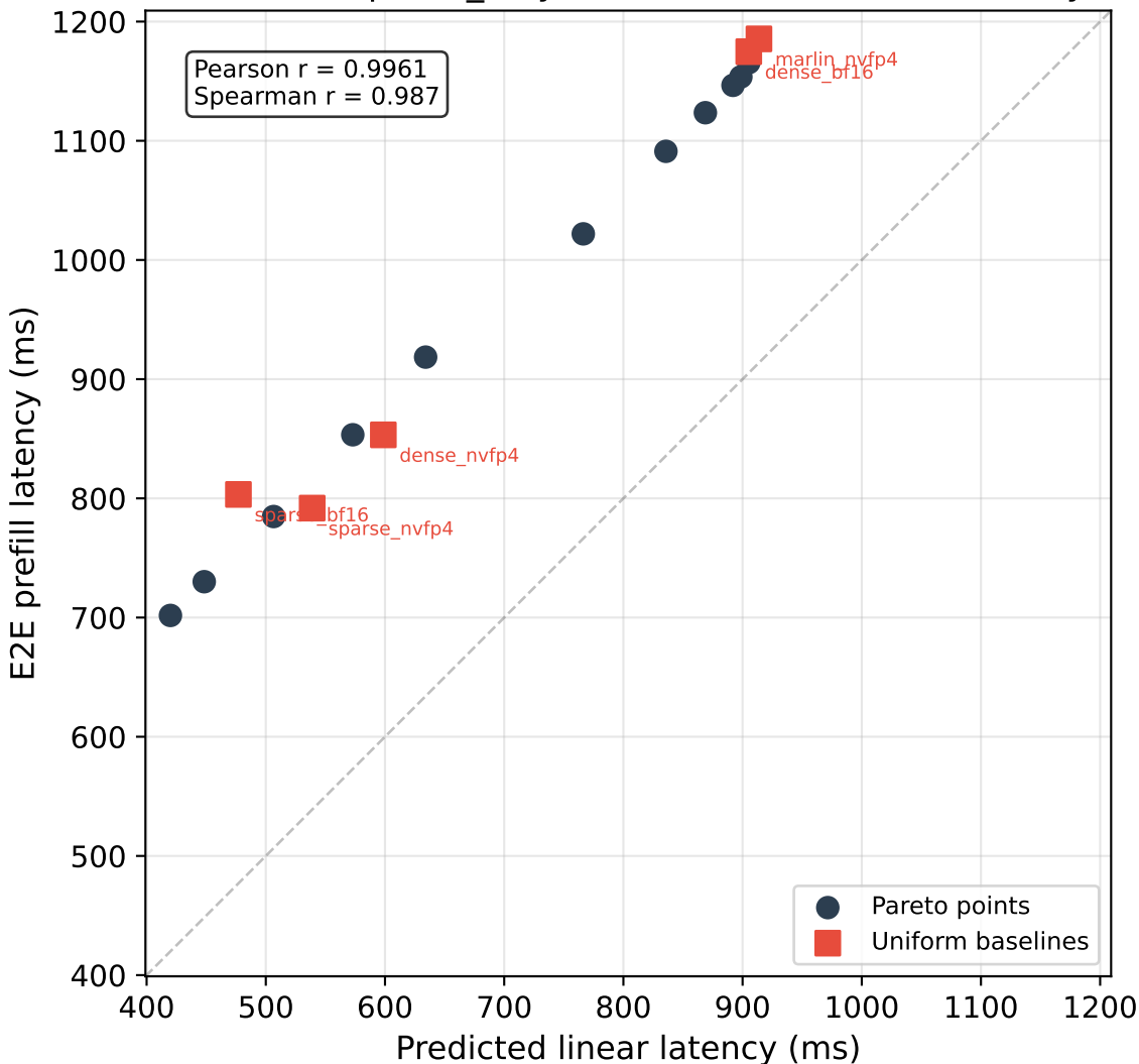
Llama2-7B prefill_only: Predicted vs real E2E latency
