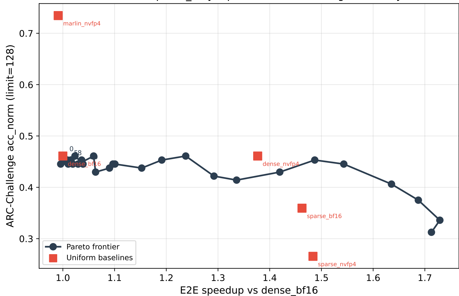
Llama2-7B prefill_only: Speed vs ARC-Challenge accuracy
