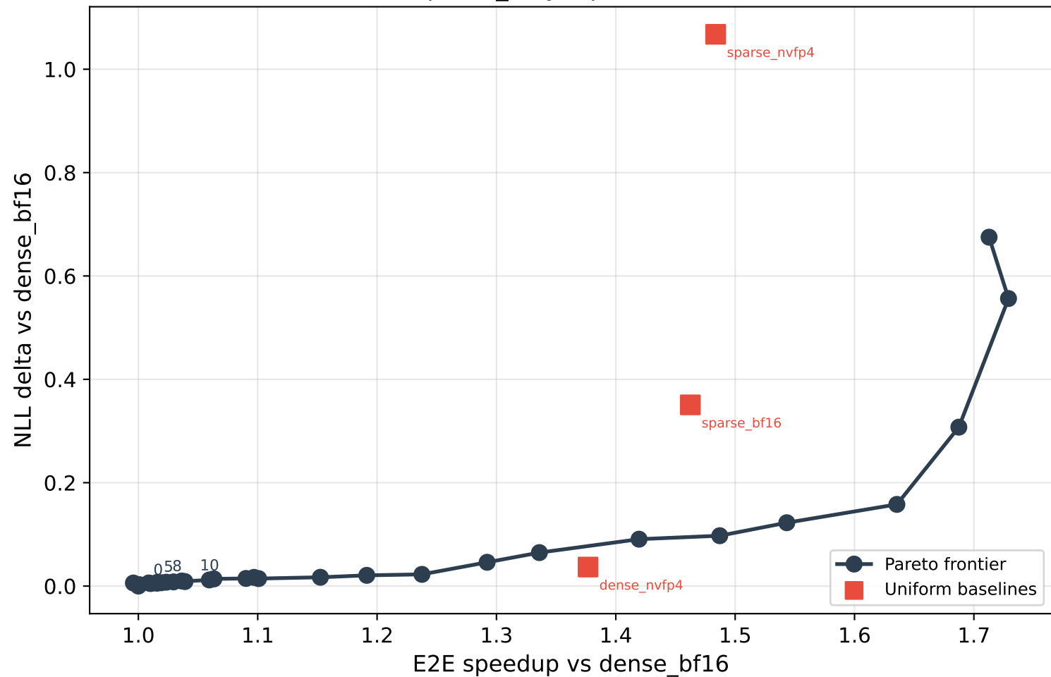
Llama2-7B prefill_only: Speed vs NLL trade-off
