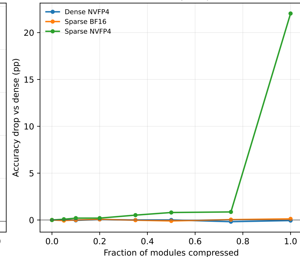
Measured accuracy-drop context
