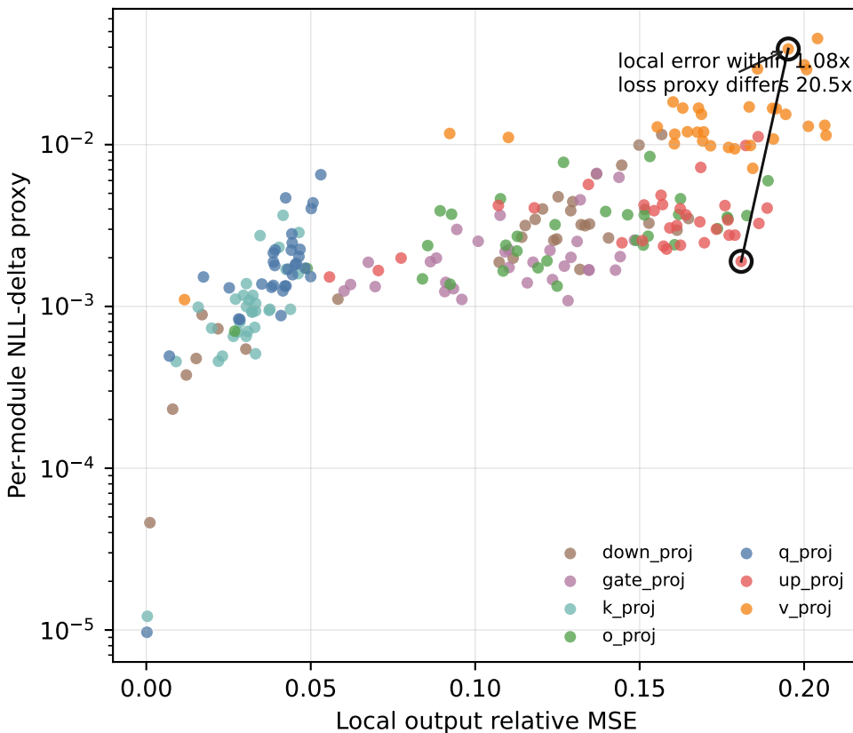
Same method, close local error
