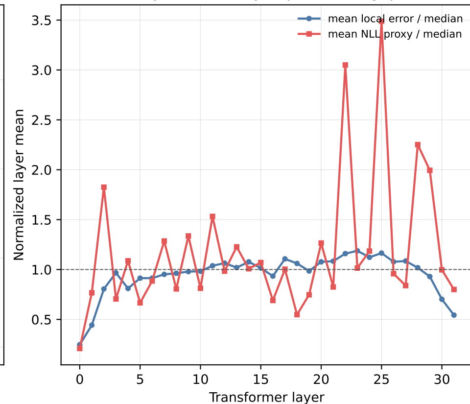
Layer sensitivity expands the gap
