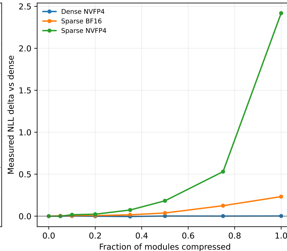
Measured full-model loss context
