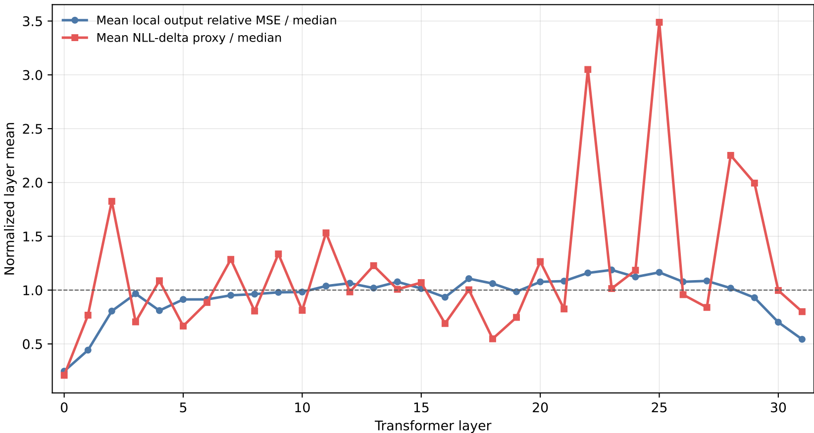
FakeVLM Sparse NVFP4: layer sensitivity expands the loss gap
