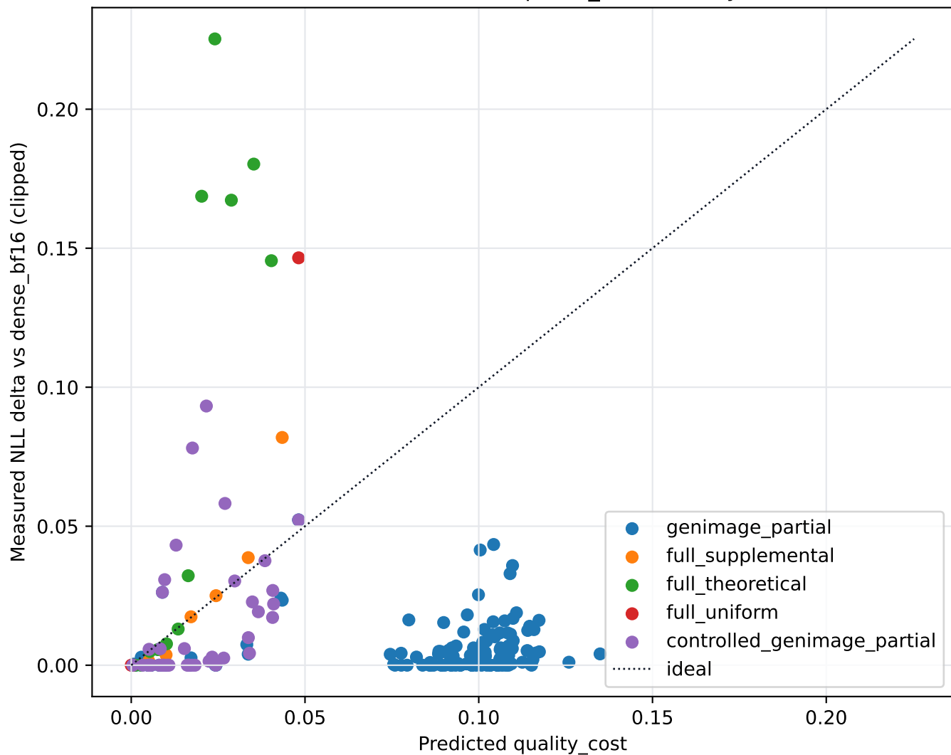
Predicted vs Measured sparse_bf16 Quality Cost
