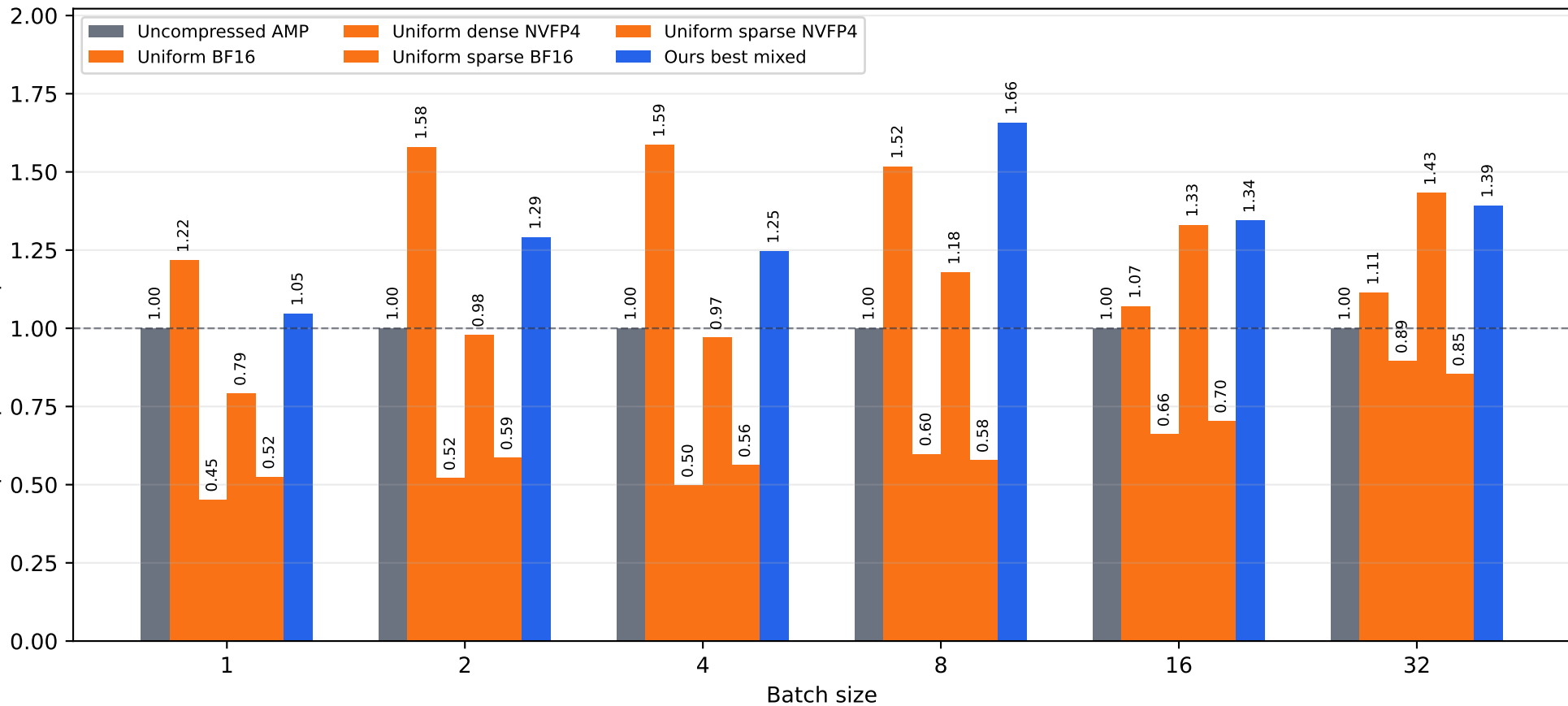
Speedup vs uncompressed AMP
