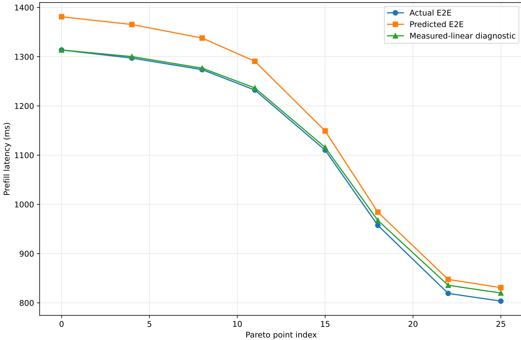
FakeVLM E2E prediction comparison: batch 16
