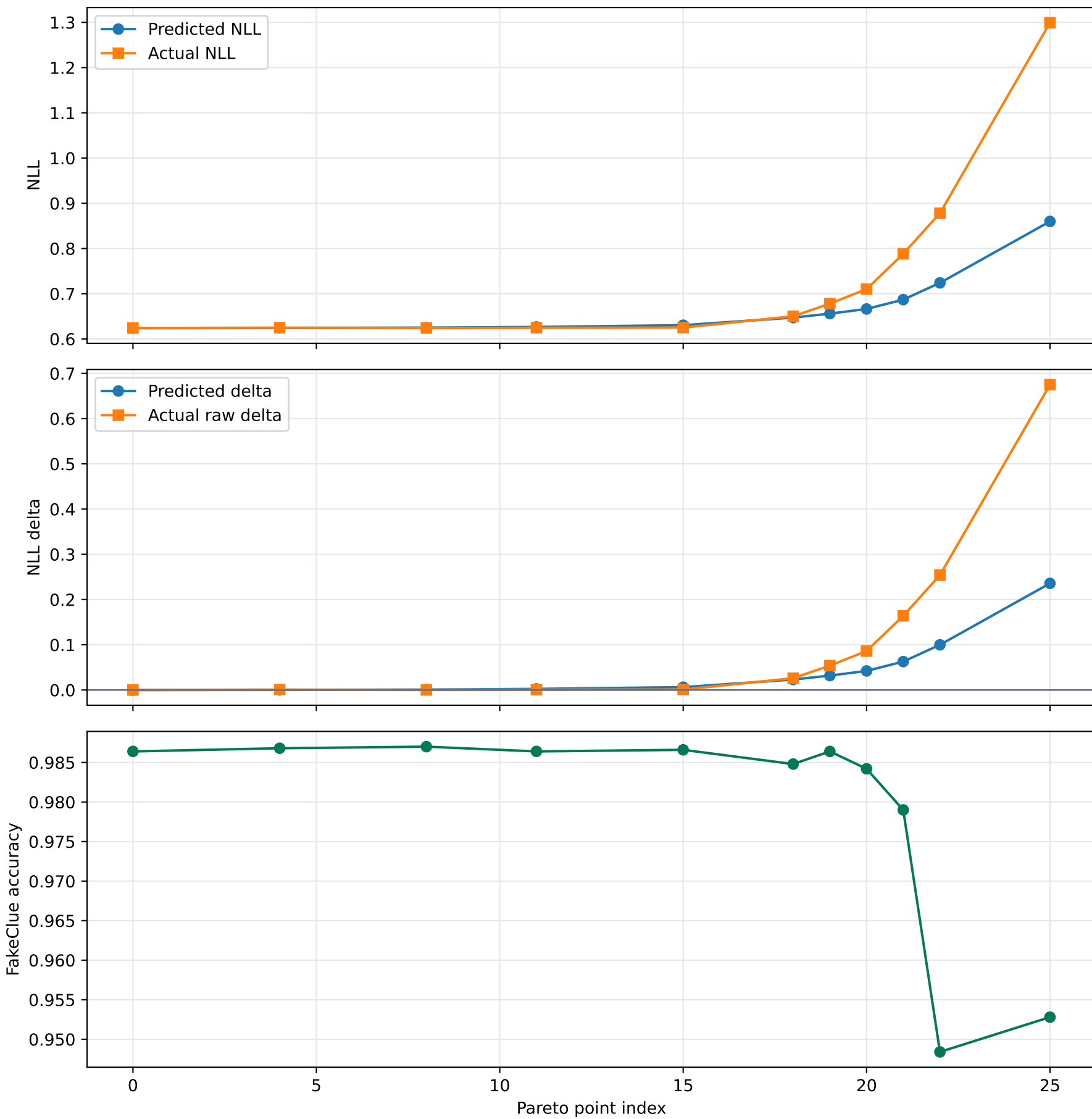
FakeVLM quality prediction and downstream result: batch 16
