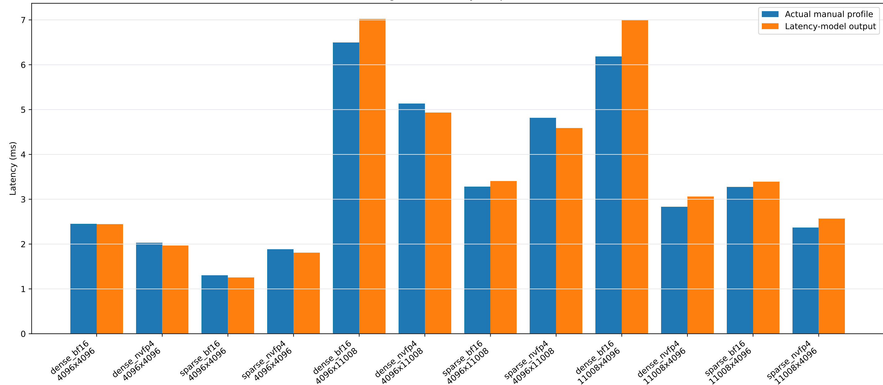
FakeVLM single-linear latency comparison: batch 16
