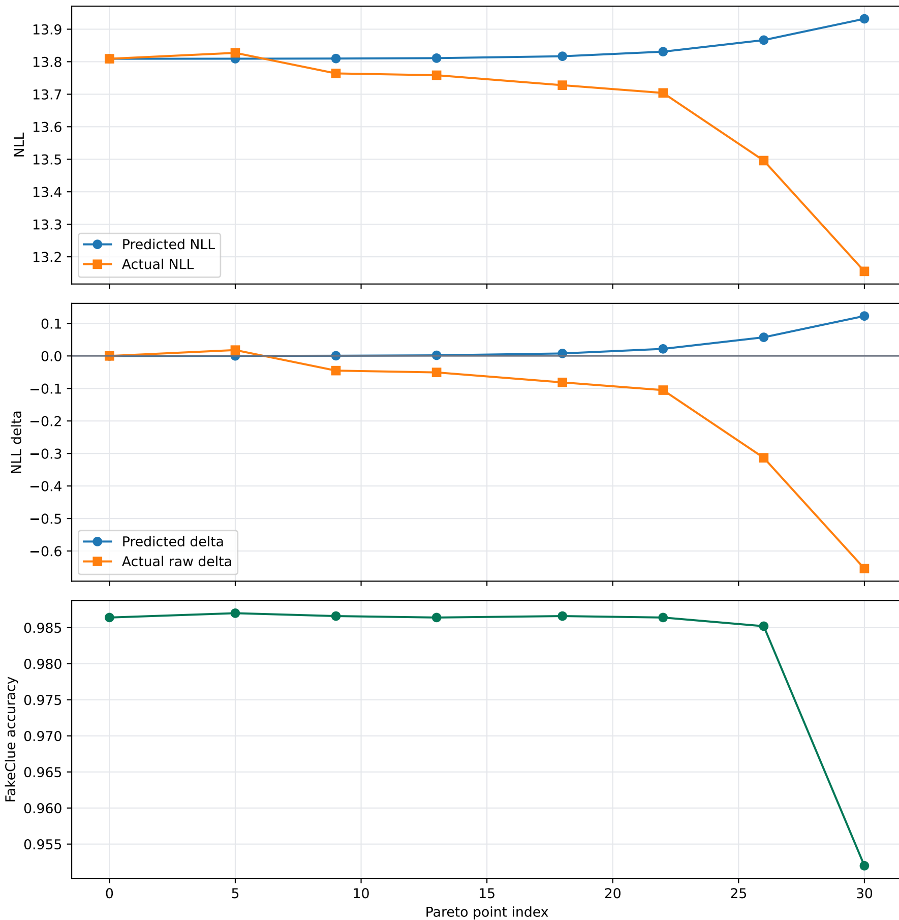
FakeVLM quality prediction and downstream result: batch 4
