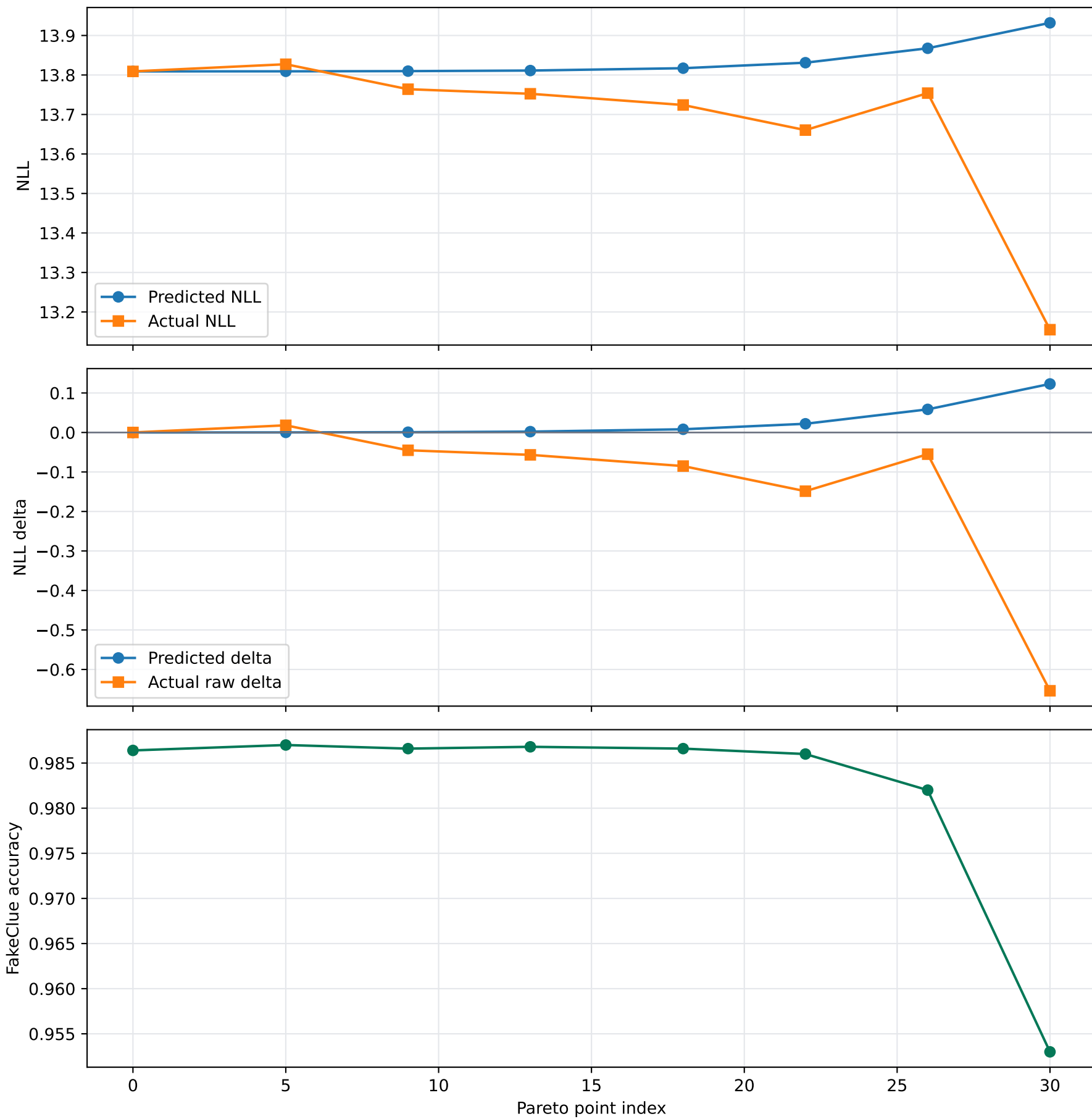
FakeVLM quality prediction and downstream result: batch 8
