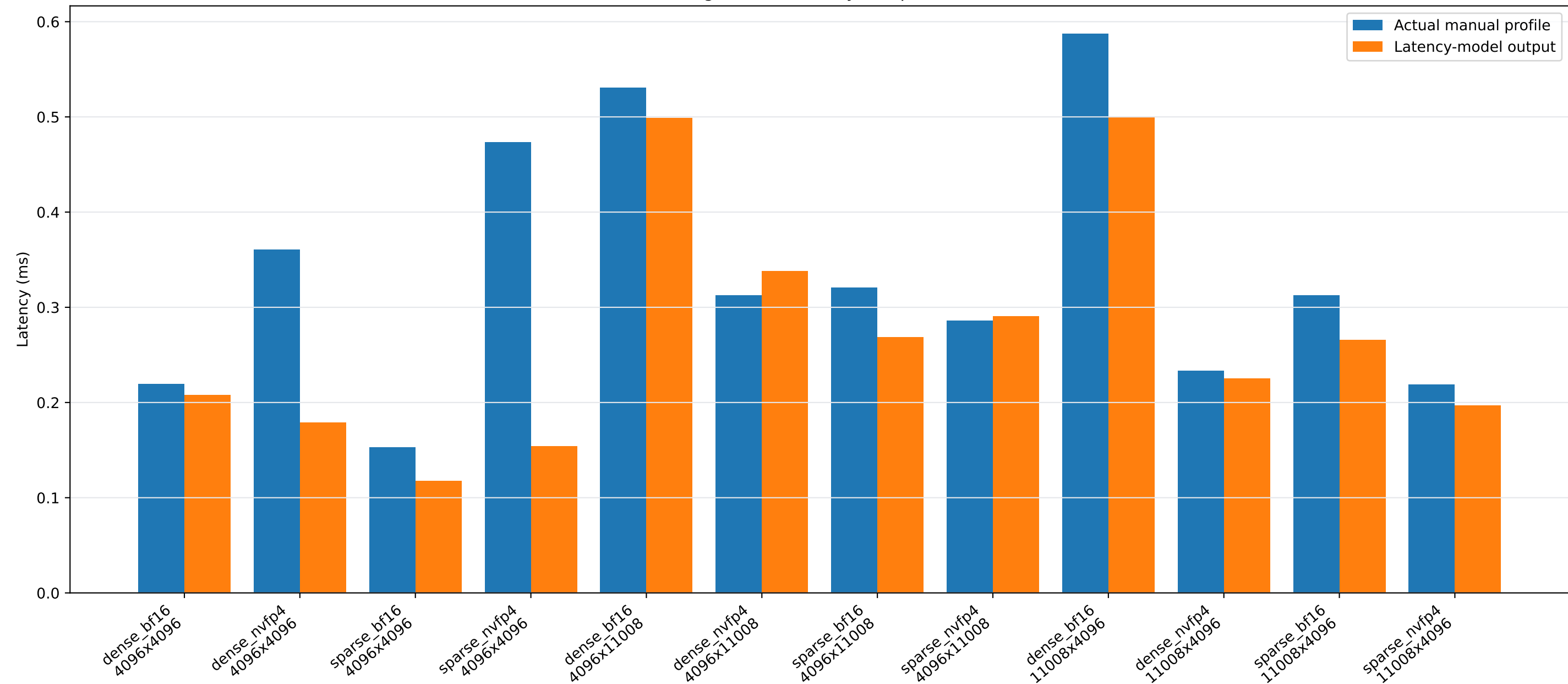
FakeVLM single-linear latency comparison: batch 1
