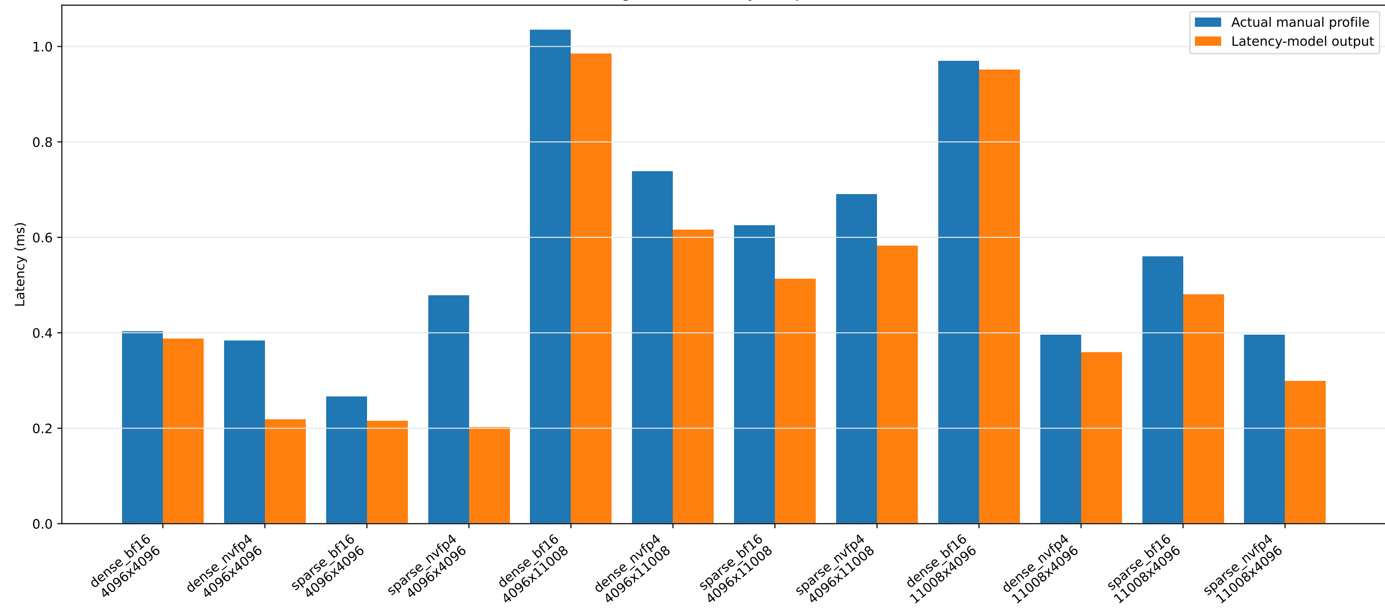
FakeVLM single-linear latency comparison: batch 2
