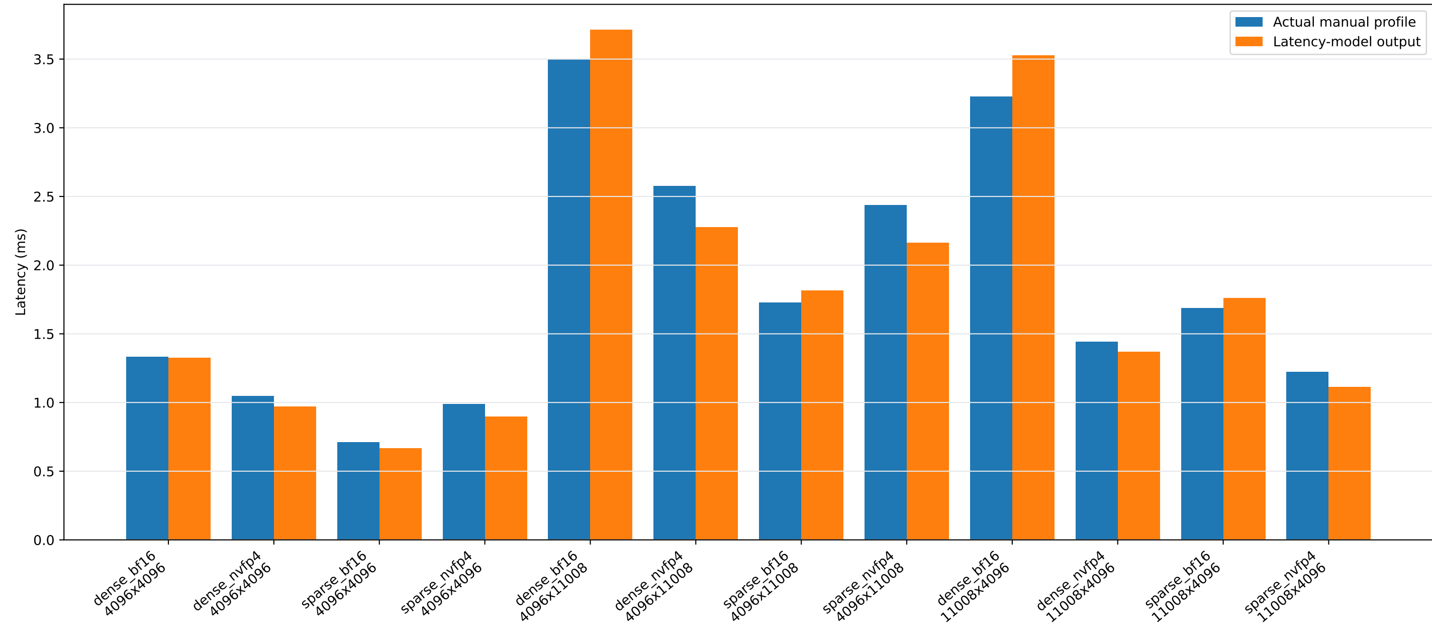
FakeVLM single-linear latency comparison: batch 8
