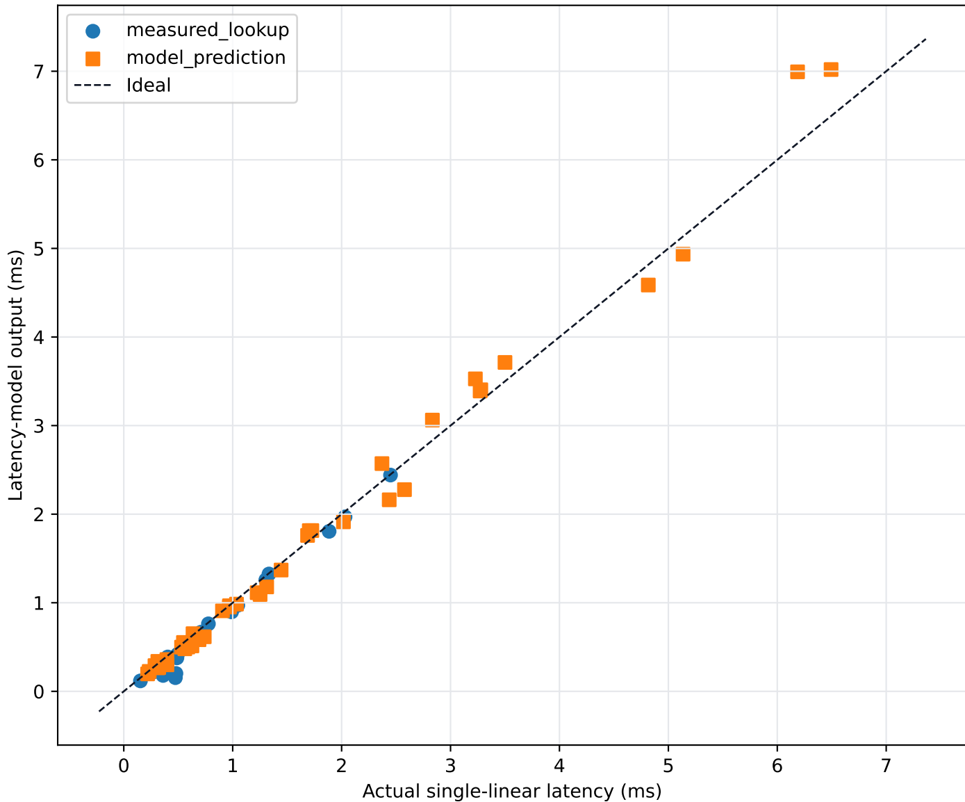
FakeVLM single-linear predicted vs actual latency
