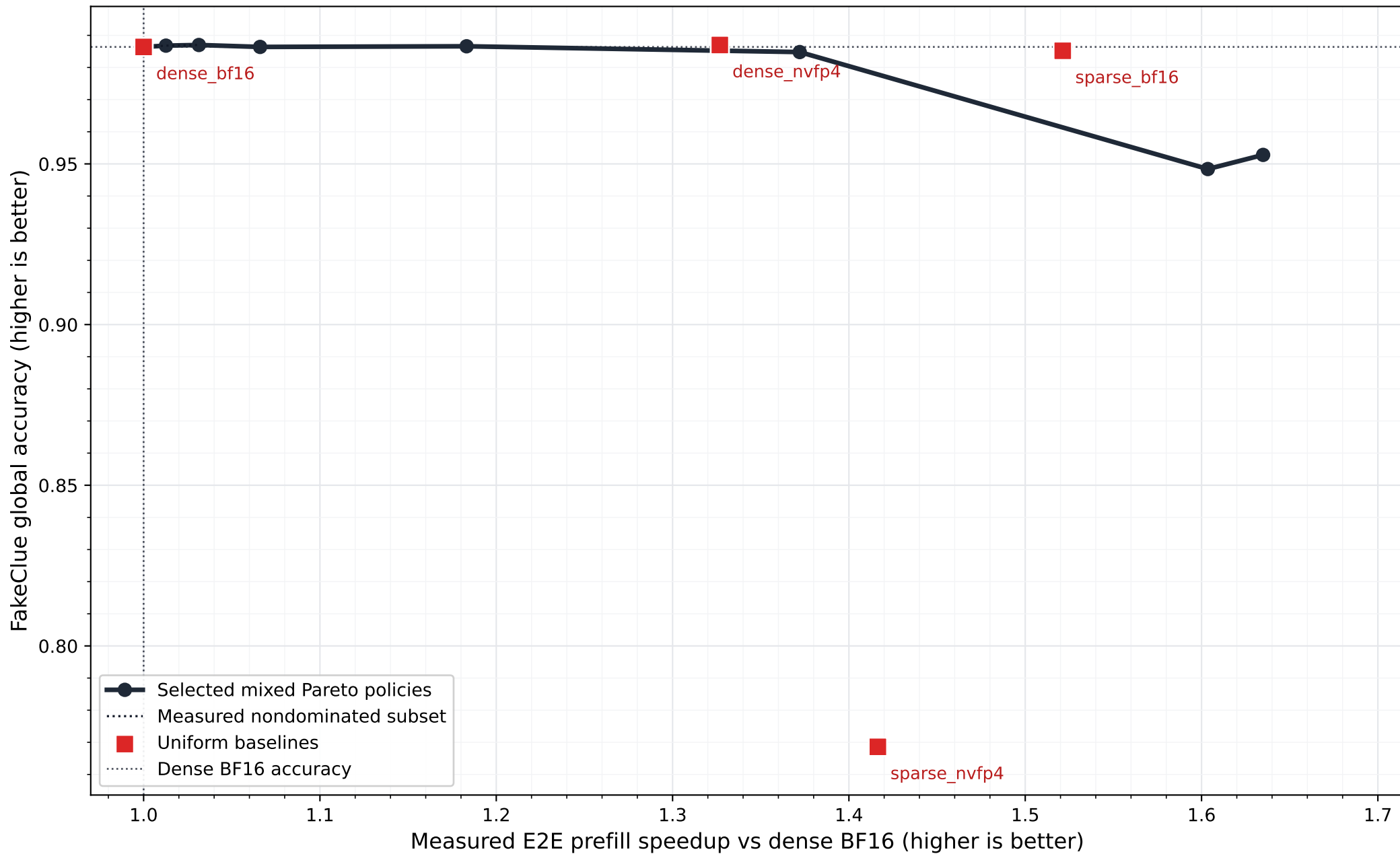
FakeVLM Prefill Pareto vs Uniform Baselines: Batch Size 16
