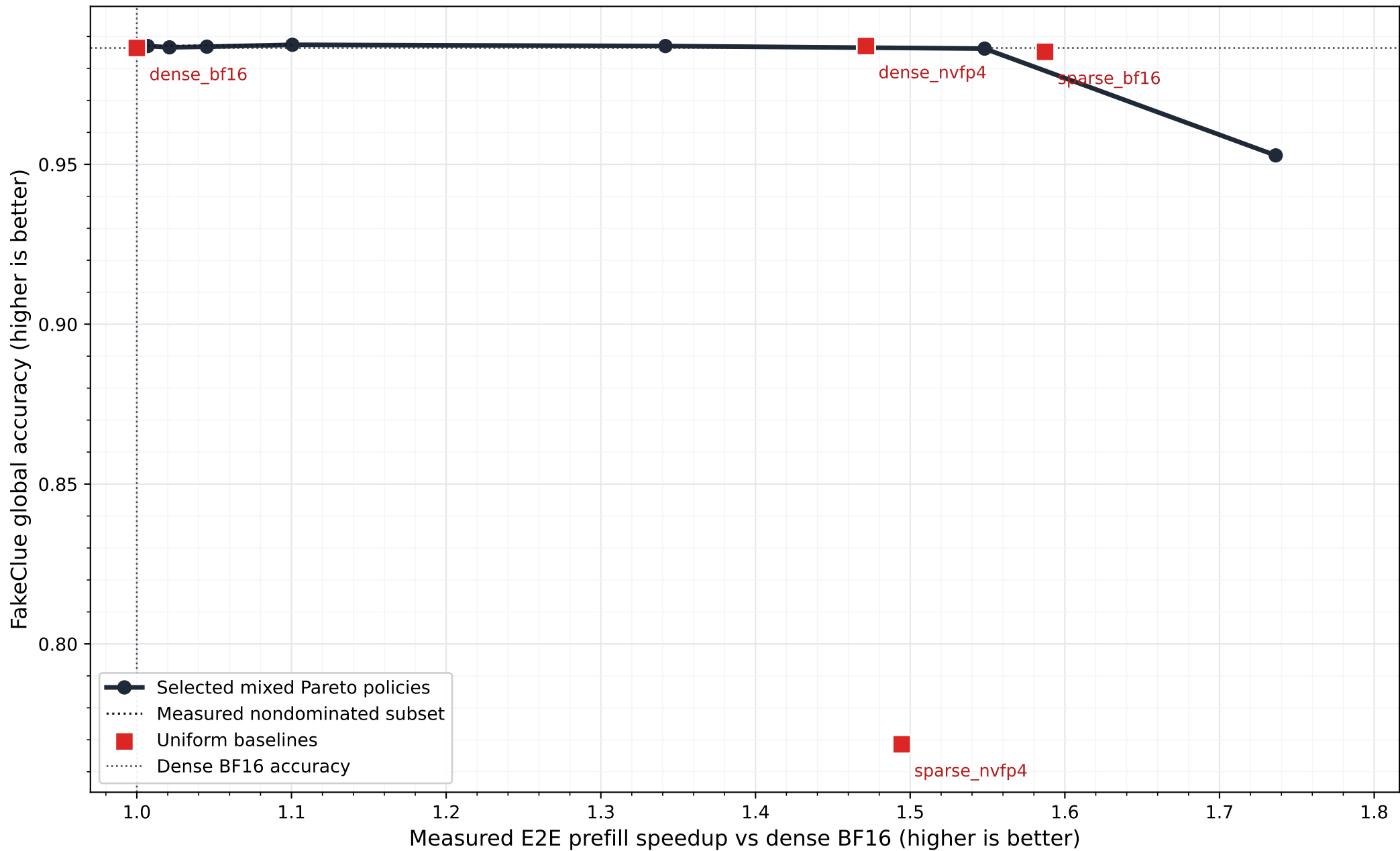
FakeVLM Prefill Pareto vs Uniform Baselines: Batch Size 1
