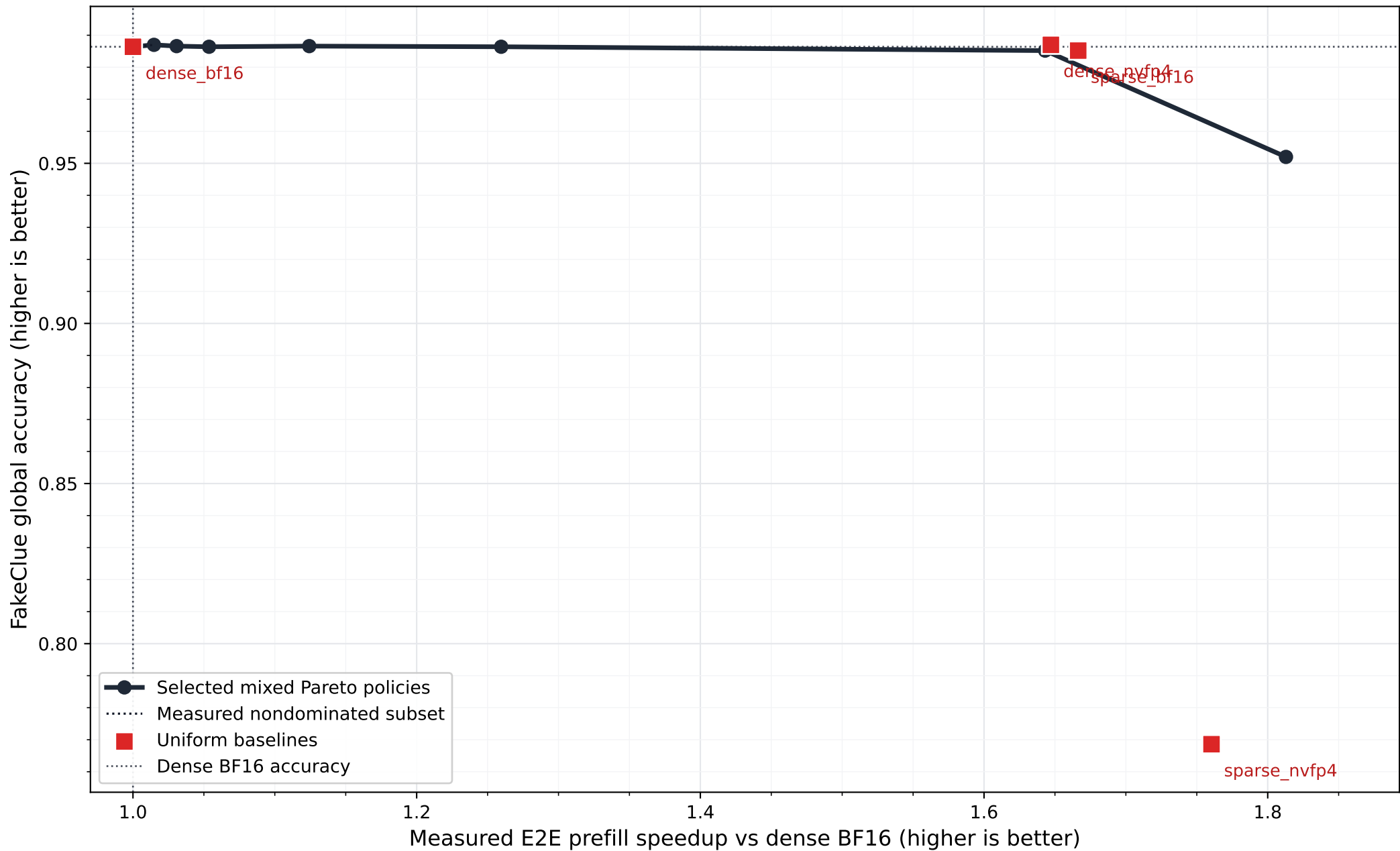
FakeVLM Prefill Pareto vs Uniform Baselines: Batch Size 4
