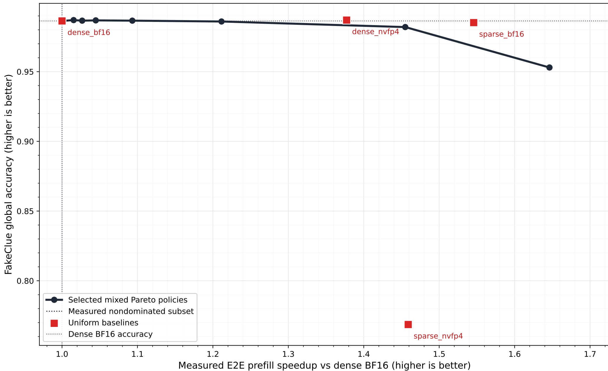
FakeVLM Prefill Pareto vs Uniform Baselines: Batch Size 8
