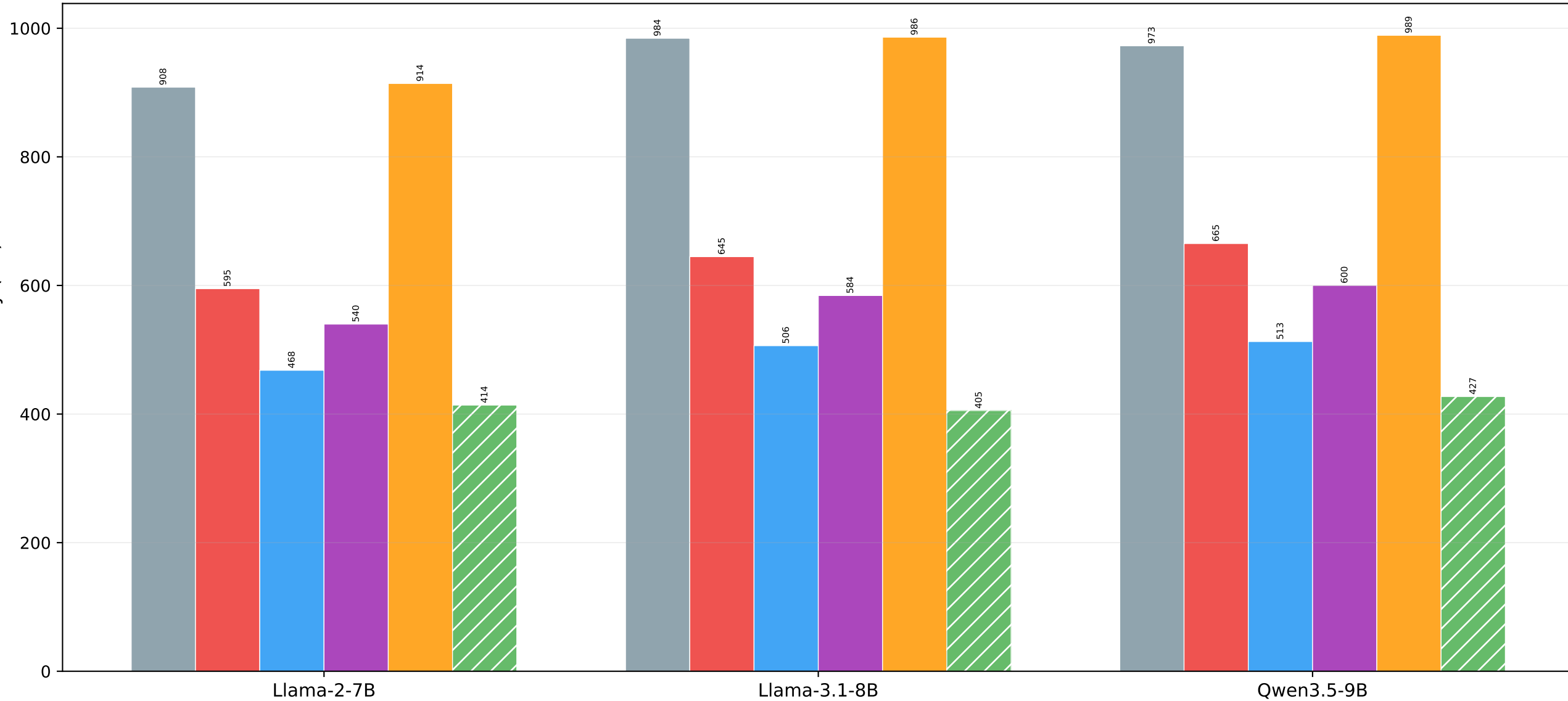
Pure Prefill Latency: batch size=16, input tokens=1024, M=16384 | GPU: NVIDIA RTX 5090 32GB
