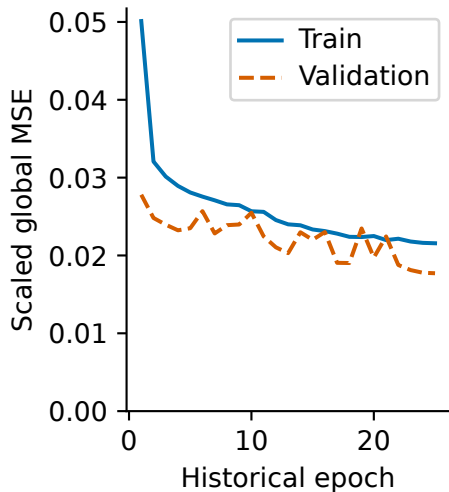
(a) NIST TCN seed 42
