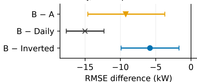
(j) NIST / power-active
