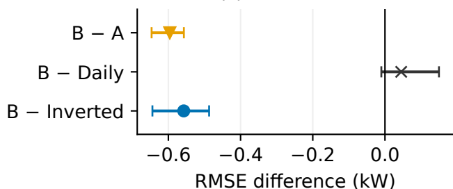
(e) Qcells / full
