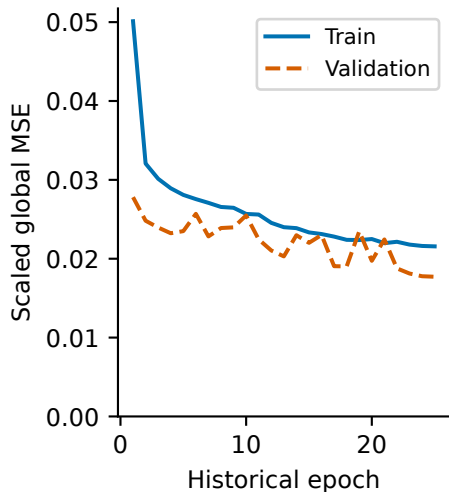
NIST TCN seed 42
