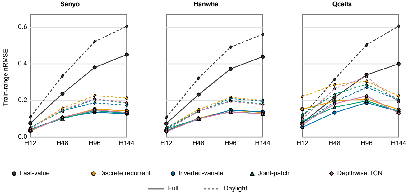
FIG. 3. Primary Train-range nRMSE across horizon and array. Solid lines denote full-timeline evaluation and dashed lines denote daylight evaluation. Every point within a panel uses model-matched horizon-specific origins and masks.
