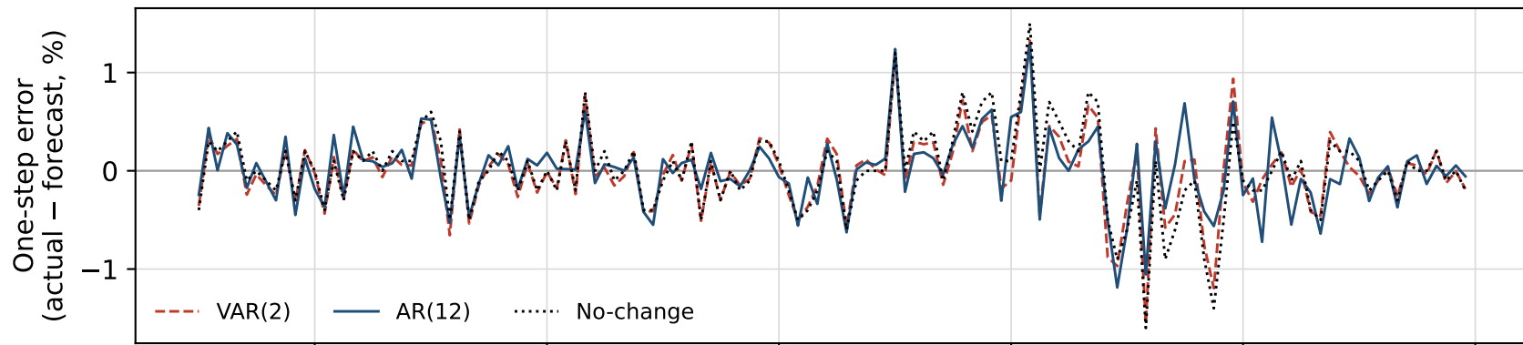
(a) forecast errors over time
