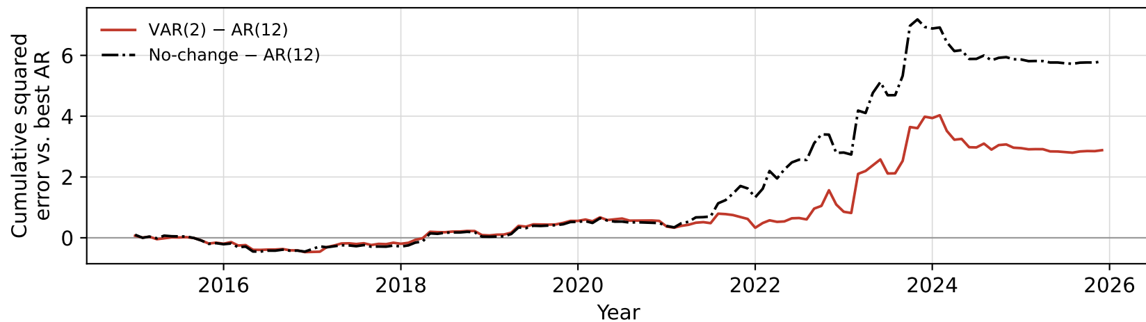
(b) running verdict: above 0 \Rightarrow AR(12) more accurate
