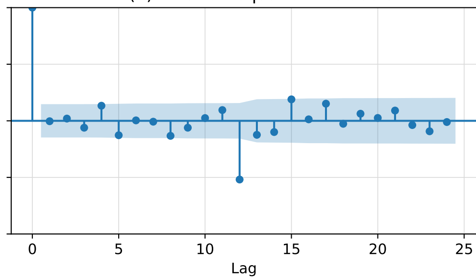
VAR(2) inflation-equation residuals
