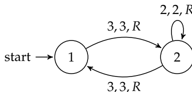
Figure 32.2: A standard Even machine
