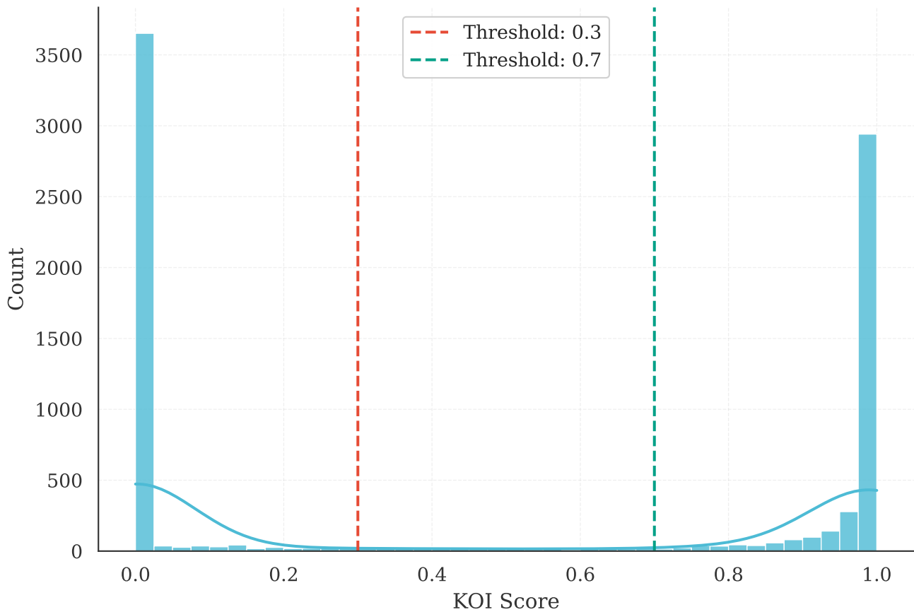
Distribution of KOI Score
