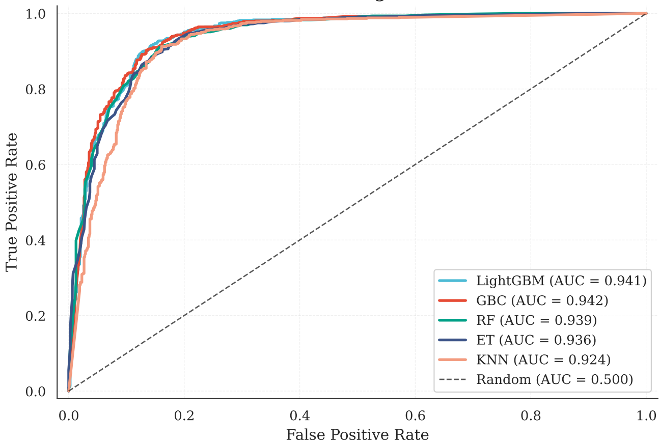
ROC Curves — Original Features
